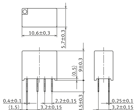
External dimensions
