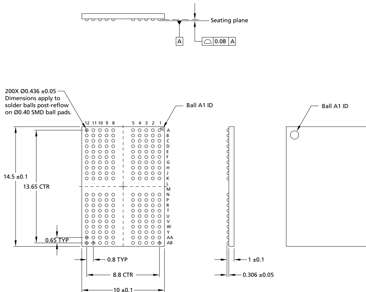
Figure 15: 200-Ball TFBGA – 10mm x 14.5mm x 1.1mm (Package Code: FW)
