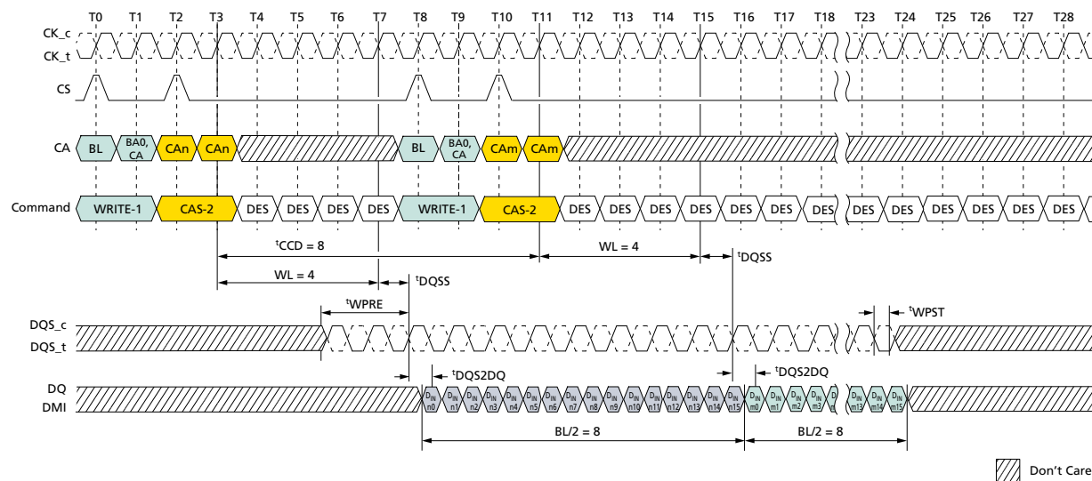
Figure 64: Seamless WRITE: t_{CCD} = \text{MIN} , 0.5n\text{CK} Postamble
