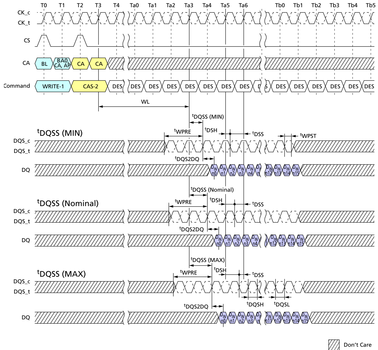
Figure 40: Write Timing
