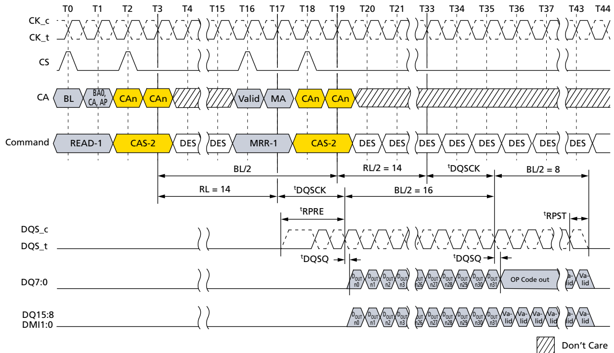
Figure 104: READ-to-MRR Timing
