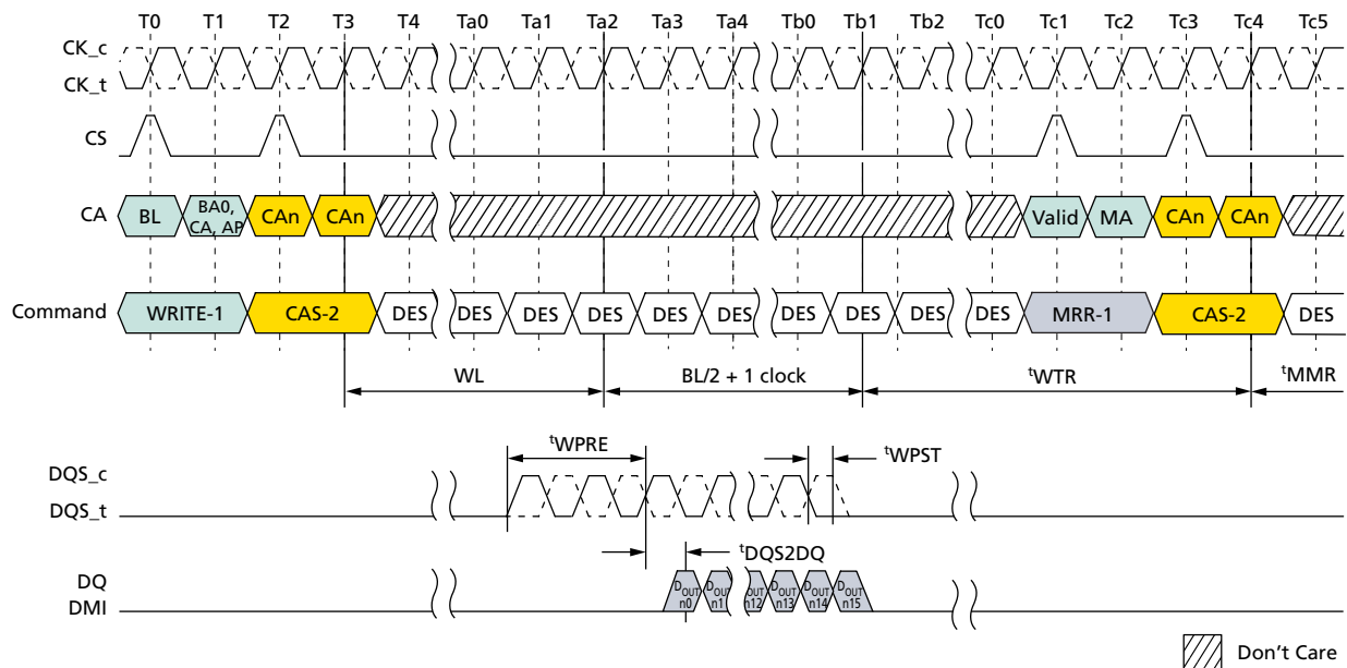
Figure 105: WRITE-to-MRR Timing
