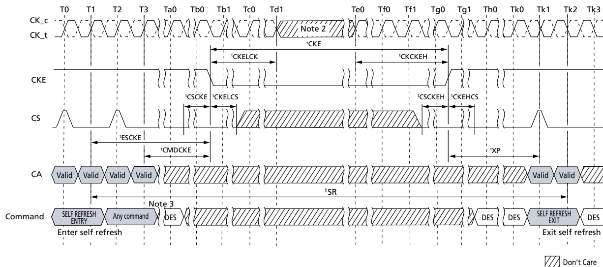
Figure 89: Self Refresh Entry/Exit Timing with Power-Down Entry/Exit
