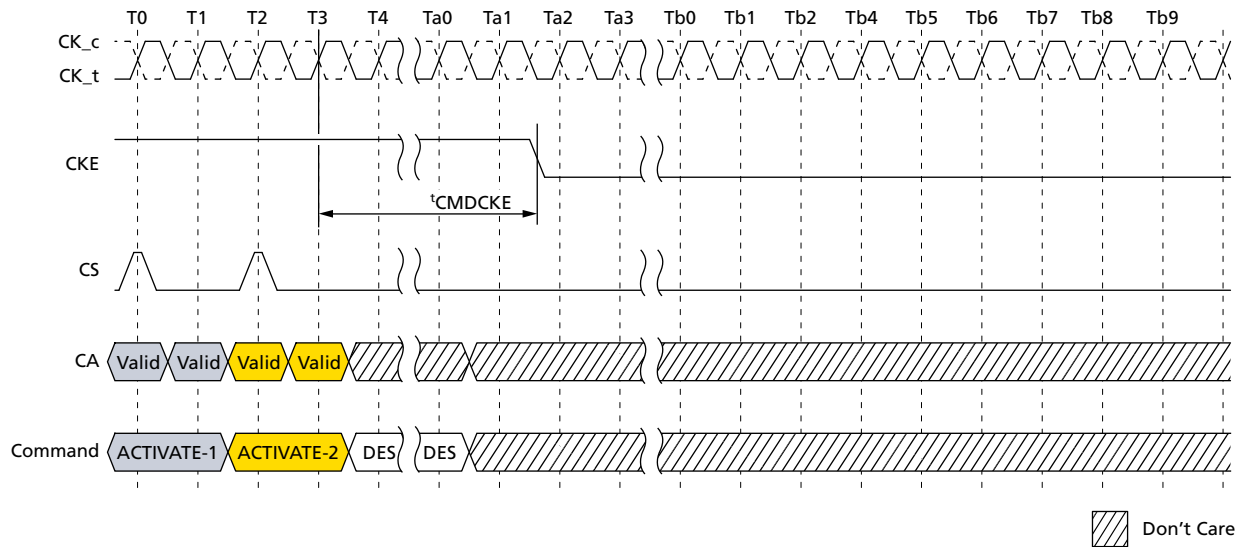
Figure 98: ACTIVATE Command to Power-Down Entry
