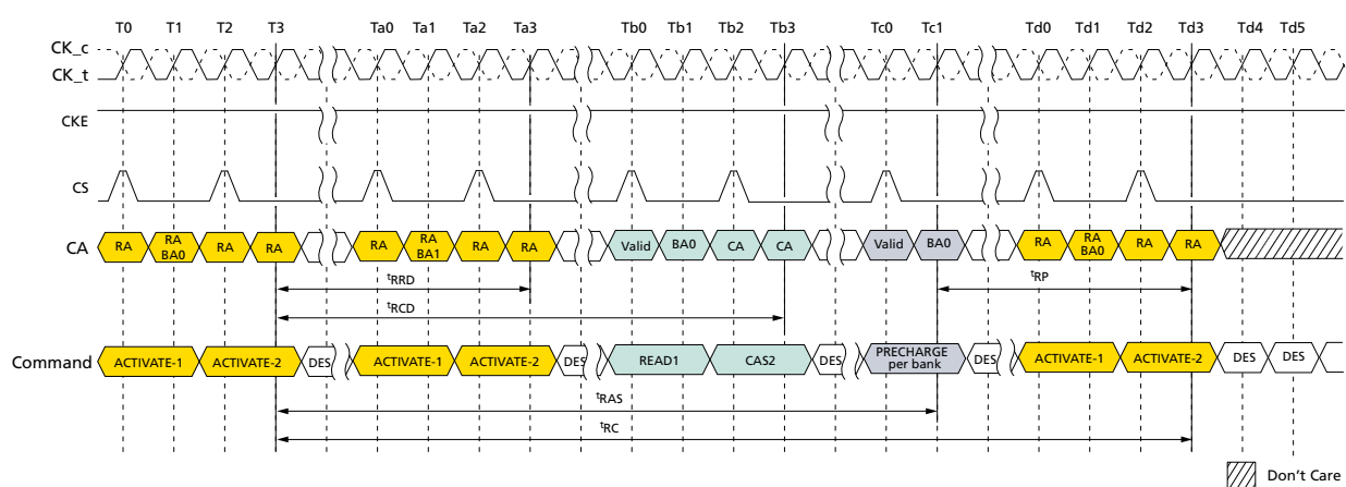
Figure 24: ACTIVATE Command
