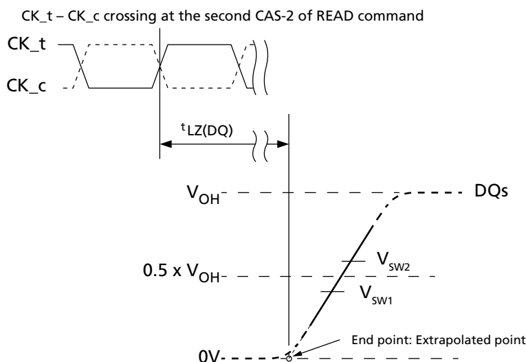
Figure 36: t_{LZ}(DQ) Method for Calculating Transitions and Endpoint
