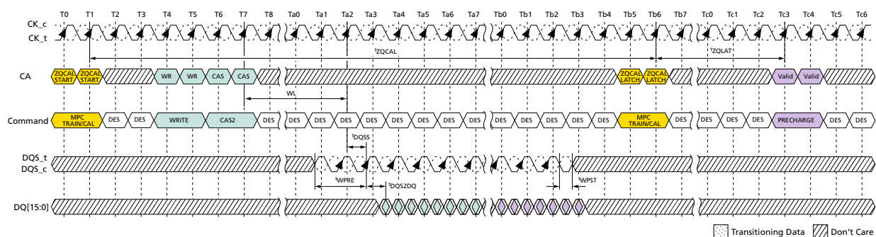
Figure 147: ZQCAL Timing
