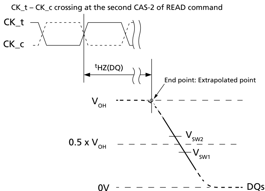
Figure 193: t_{HZ}(DQ) Method for Calculating Transitions and Endpoint
