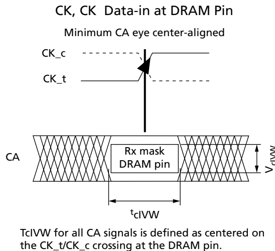
Figure 181: CA Timings at the DRAM Pins
