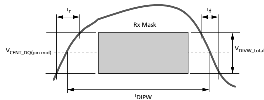
Figure 188: DQ t_{DIPW} and SRIN_dIVW Definition for Each Input Pulse
