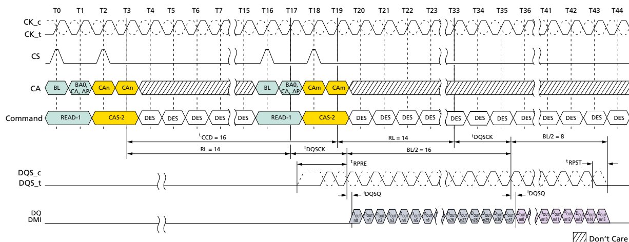
Figure 30: Burst Read Timing
