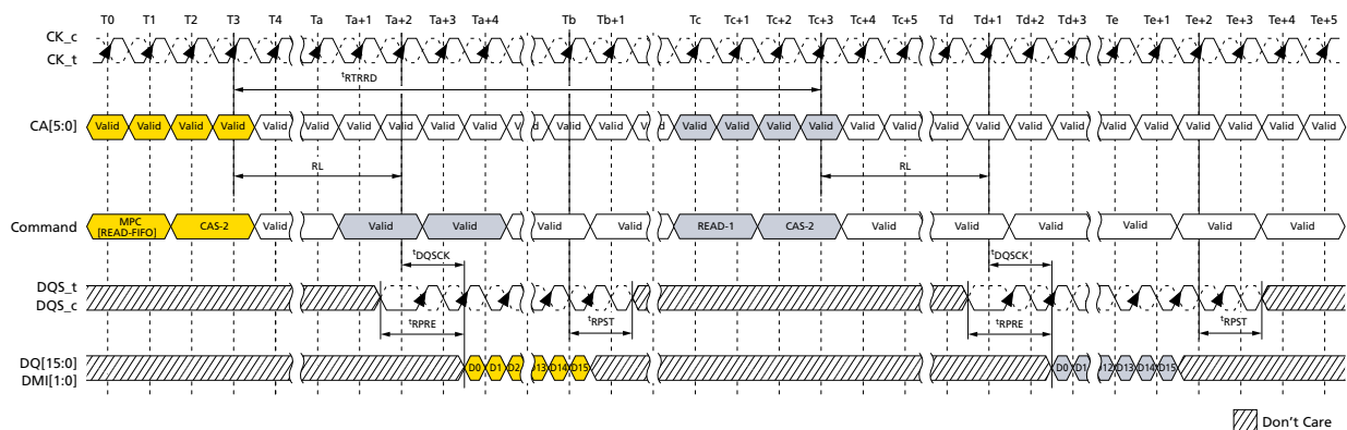
Figure 134: READ-FIFO – t_{RPRE} = \text{Toggle} , t_{RPST} = 1.5nCK
