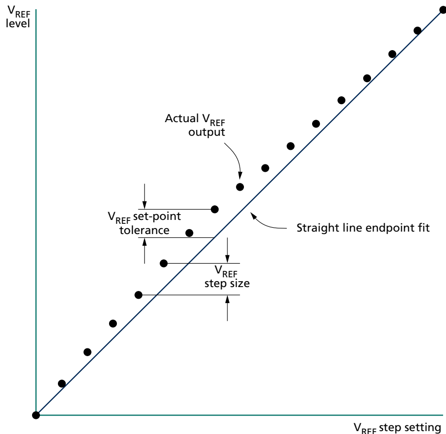
Figure 111: V_{REF} Set-Point Tolerance and Step Size
