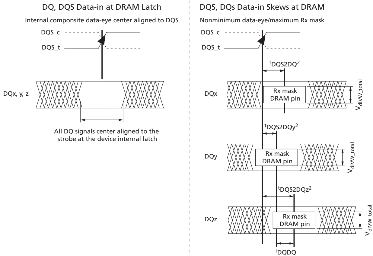
Figure 187: DQ-to-DQS t_{DQS2DQ} and t_{DQDQ}
