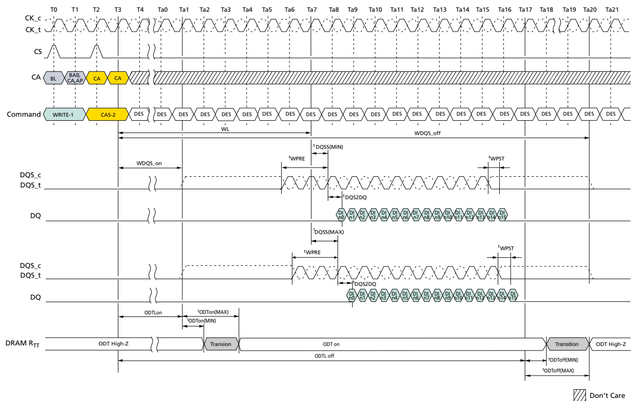
Figure 48: Burst WRITE Operation
