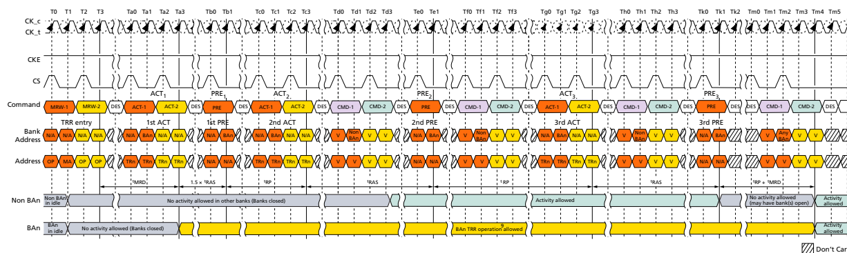
Figure 156: Target Row Refresh Mode
