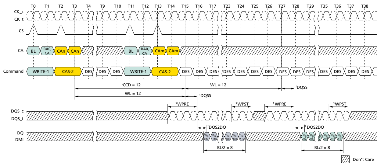
Figure 73: Consecutive WRITE: t_{\text{CCD}} = \text{MIN} + 4, 1.5n\text{CK} Postamble
