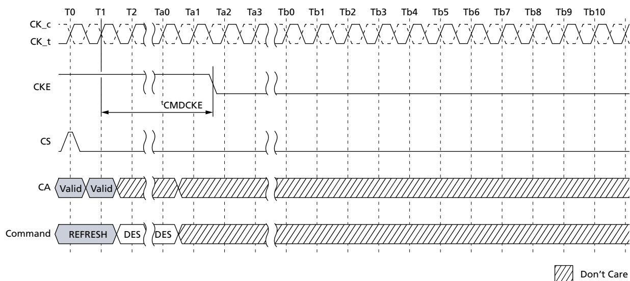
Figure 97: Refresh Entry to Power-Down Entry
