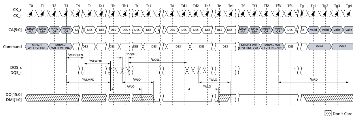
Figure 128: Write Leveling Timing – t_{DQSL}(\text{MAX})
