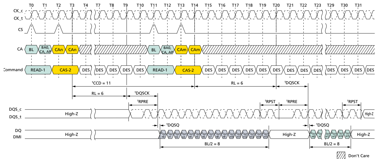
Figure 60: Consecutive READ: t_{CCD} = \text{MIN} + 3 , Preamble = Toggle, 1.5n\text{CK} Postamble
