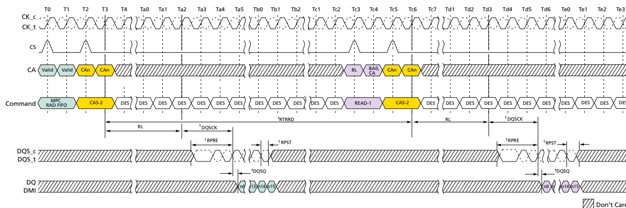
Figure 140: MPC[READ-FIFO] to Read Timing
