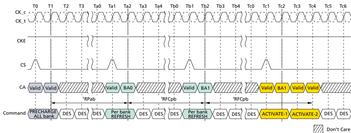
Figure 83: Per-Bank REFRESH Operation
