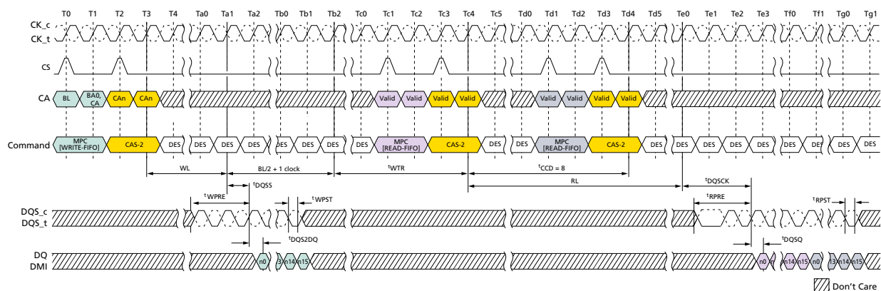
Figure 139: MPC[WRITE-FIFO]-to-MPC[READ-FIFO] Timing
