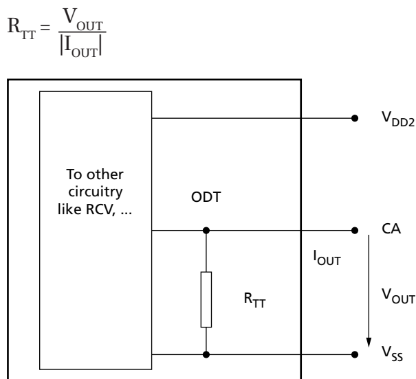
Figure 152: ODT for CA
