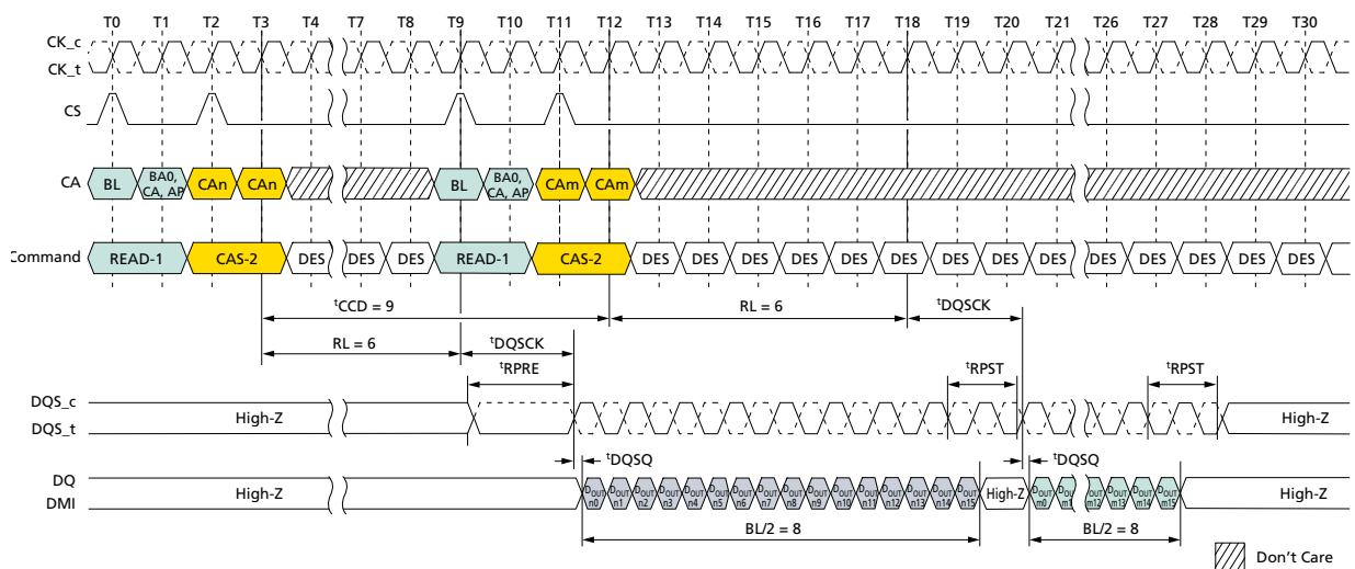
Figure 54: Consecutive READ: t_{CCD} = \text{MIN} + 1 , Preamble = Static, 1.5n\text{CK} Postamble
