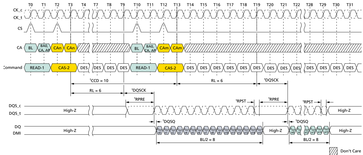
Figure 59: Consecutive READ: t_{CCD} = \text{MIN} + 2 , Preamble = Static, 0.5n\text{CK} Postamble
