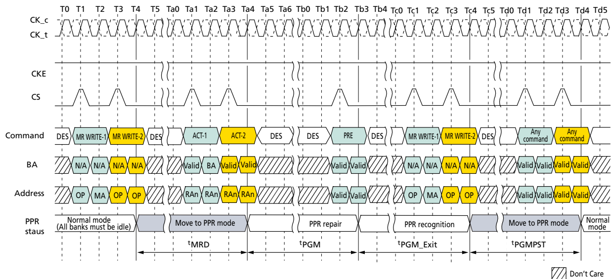
Figure 157: Post-Package Repair Timing
