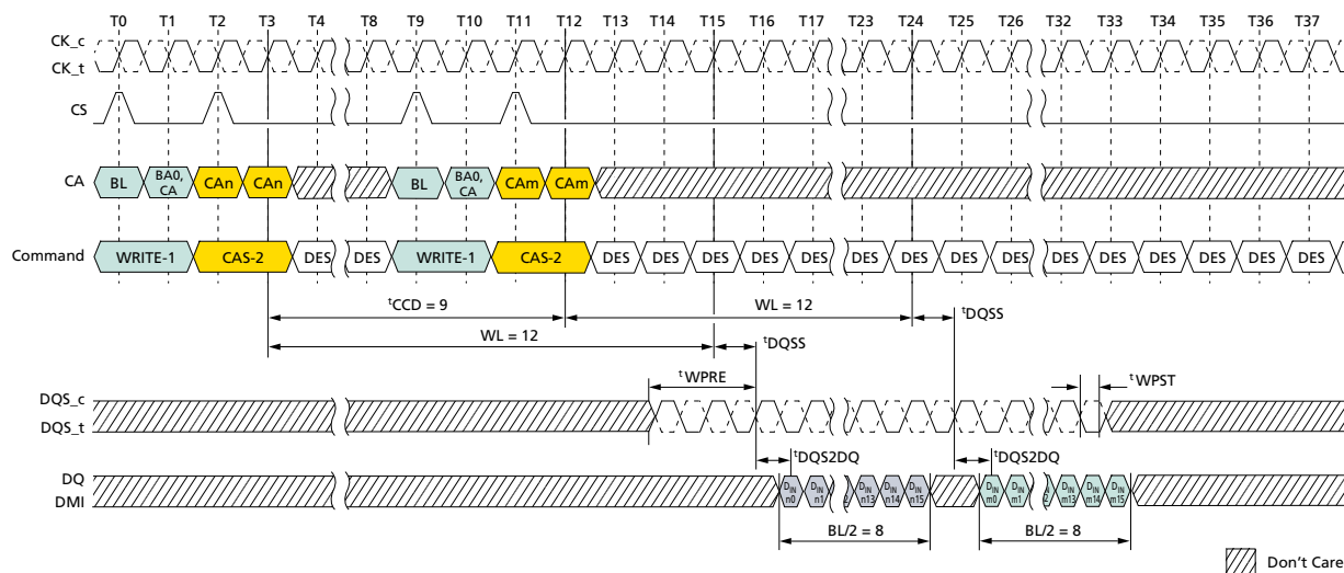
Figure 67: Consecutive WRITE: t_{CCD} = MIN + 1, 0.5nCK Postamble
