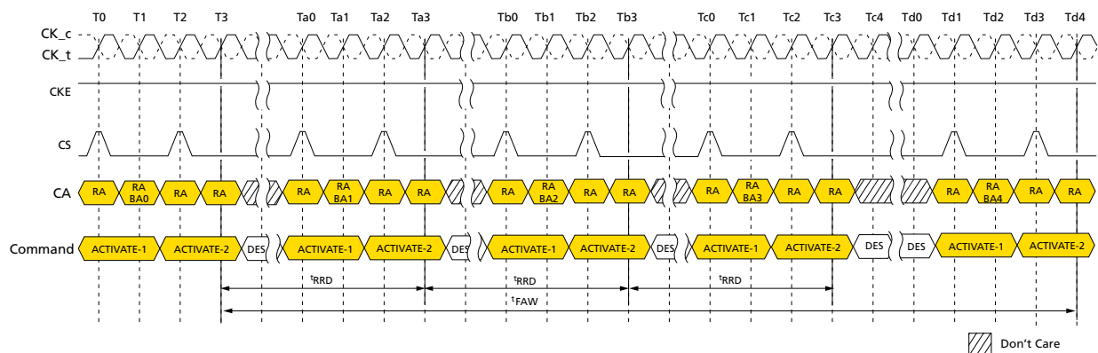
Figure 25: t_{FAW} Timing
