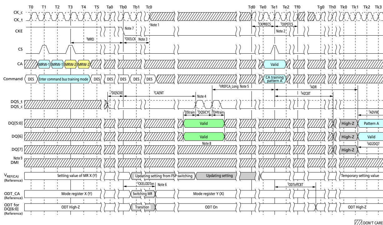
Figure 203: Entering Command Bus Training Mode and CA Training Pattern Input with V_{REF(CA)} Value Update
