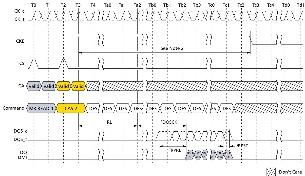
Figure 100: Mode Register Read to Power-Down Entry
