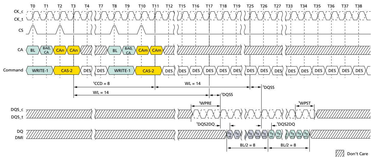
Figure 66: Seamless WRITE: t_{CCD} = \text{MIN} , 1.5nCK Postamble
