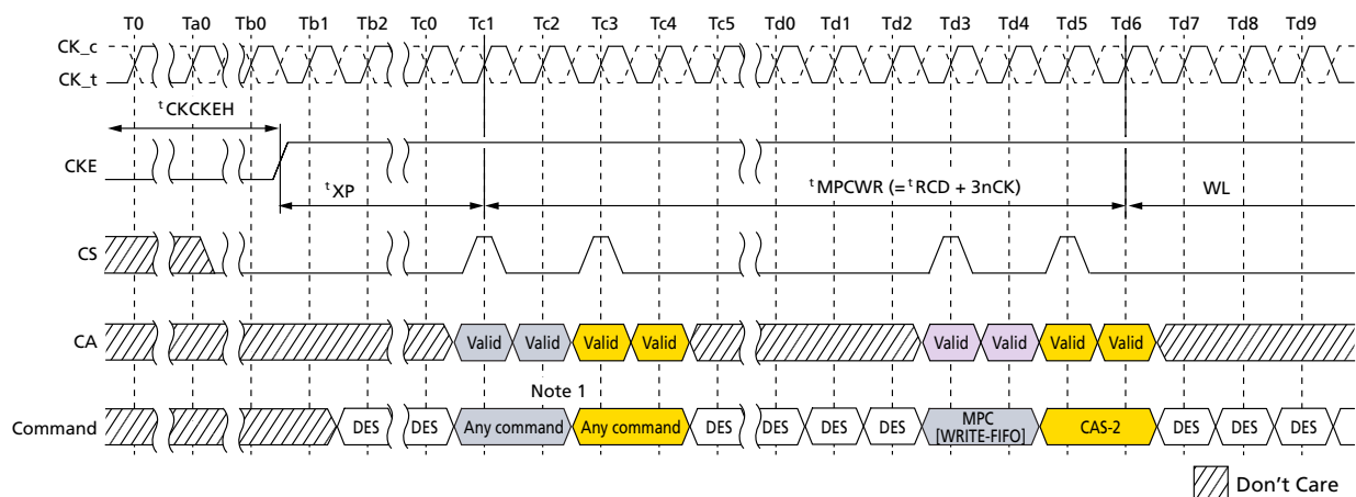
Figure 142: Power-Down Exit to MPC[WRITE-FIFO] Timing
