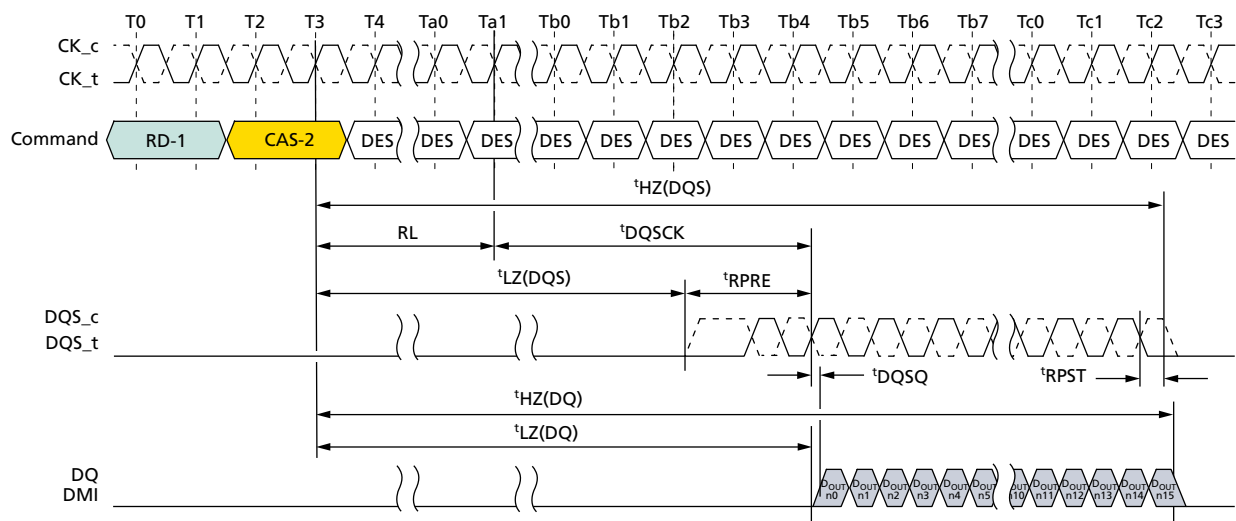
Figure 33: Read Timing
