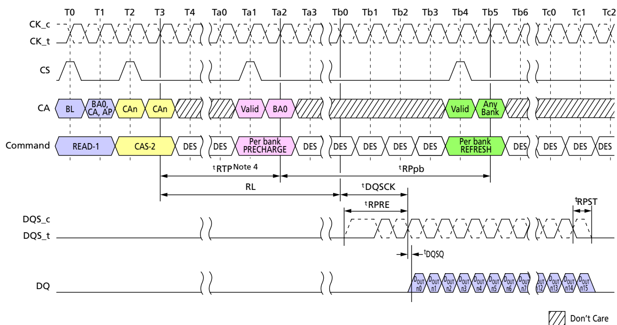
Figure 86: Burst READ Operation Followed by Per-Bank Refresh
