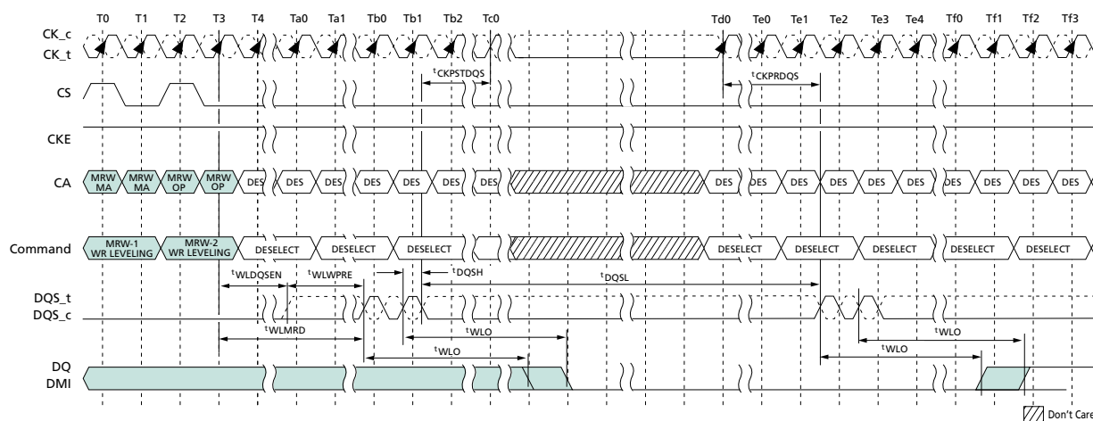
Figure 130: Clock Stop and Timing During Write Leveling
