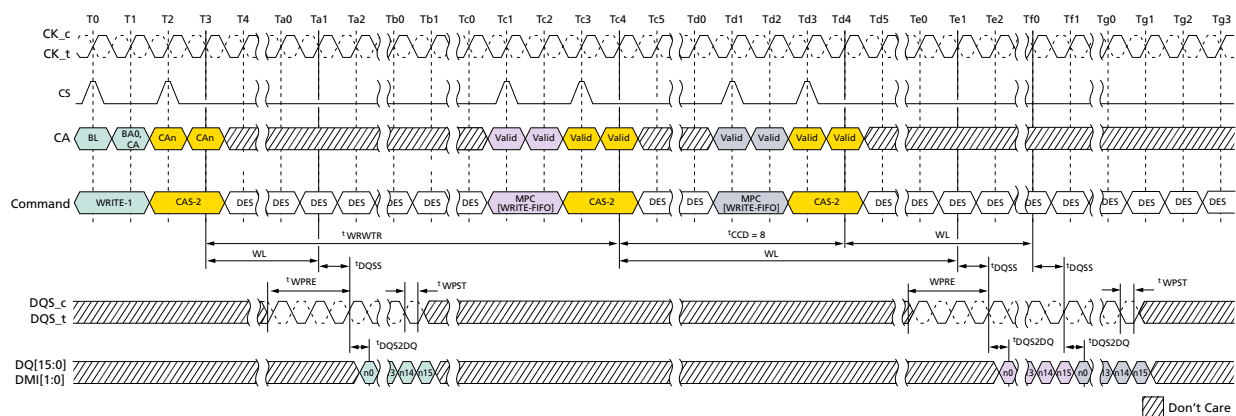
Figure 132: WRITE-FIFO – t_{WPRE} = 2nCK , t_{WPST} = 0.5nCK
