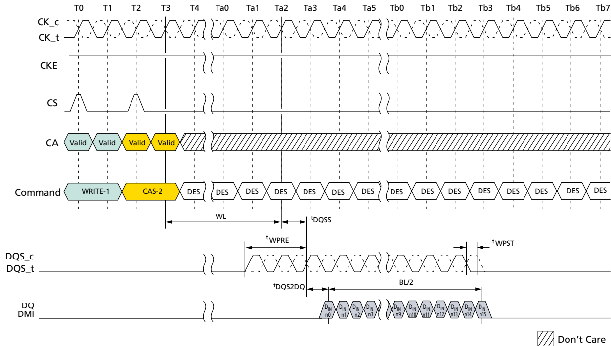
Figure 28: DQS Write Preamble and Postamble – 0.5nCK Postamble
