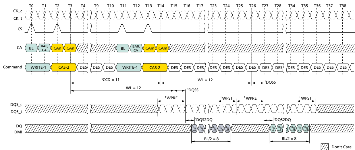
Figure 72: Consecutive WRITE: t_{CCD} = \text{MIN} + 3, 1.5n\text{CK} Postamble
