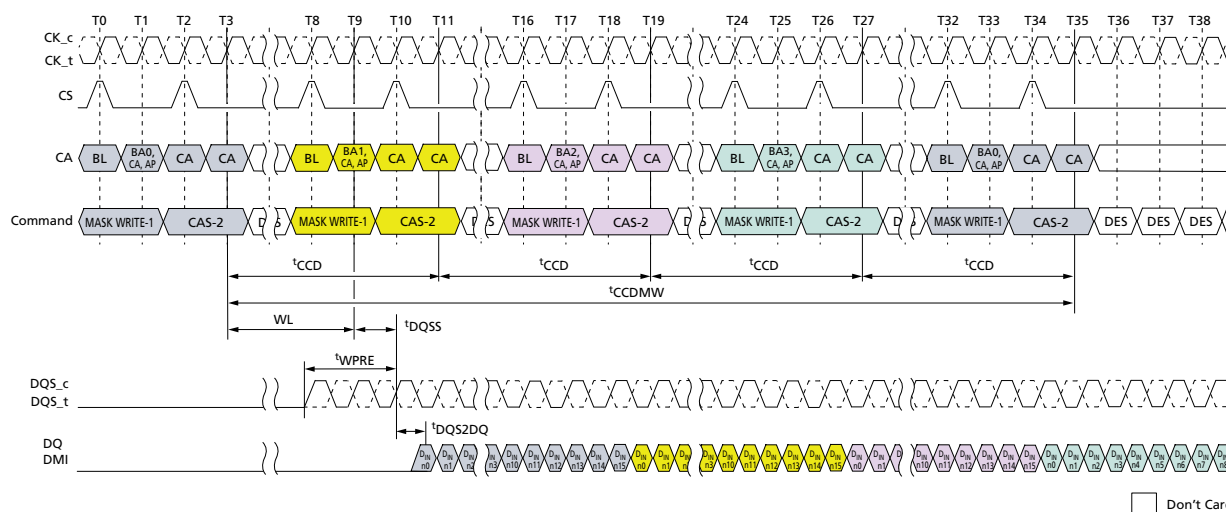
Figure 44: MASK WRITE Command – Different Bank
