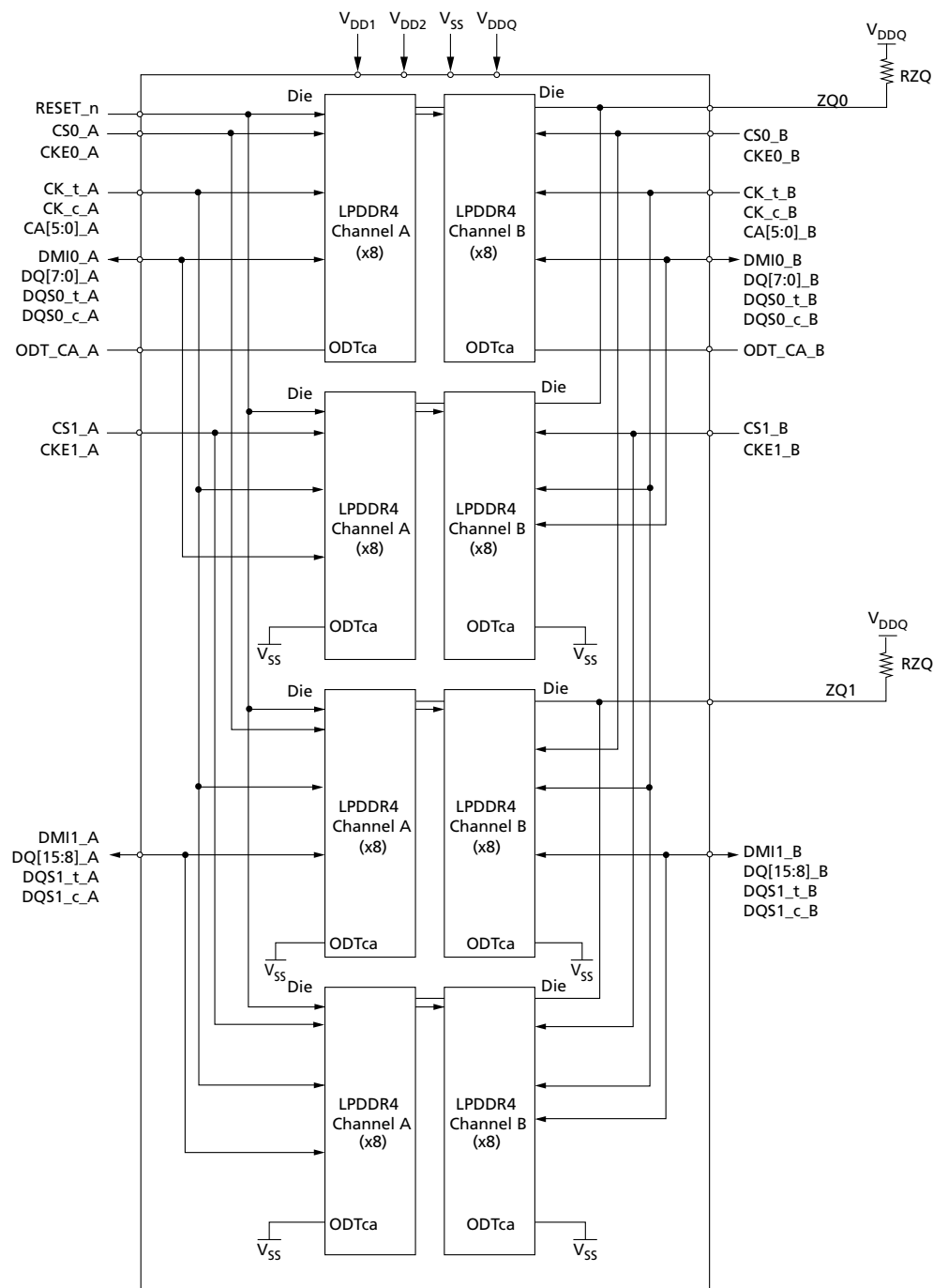
Figure 5: Eight-Die, Dual-Channel, Dual-Rank Package Block Diagram
