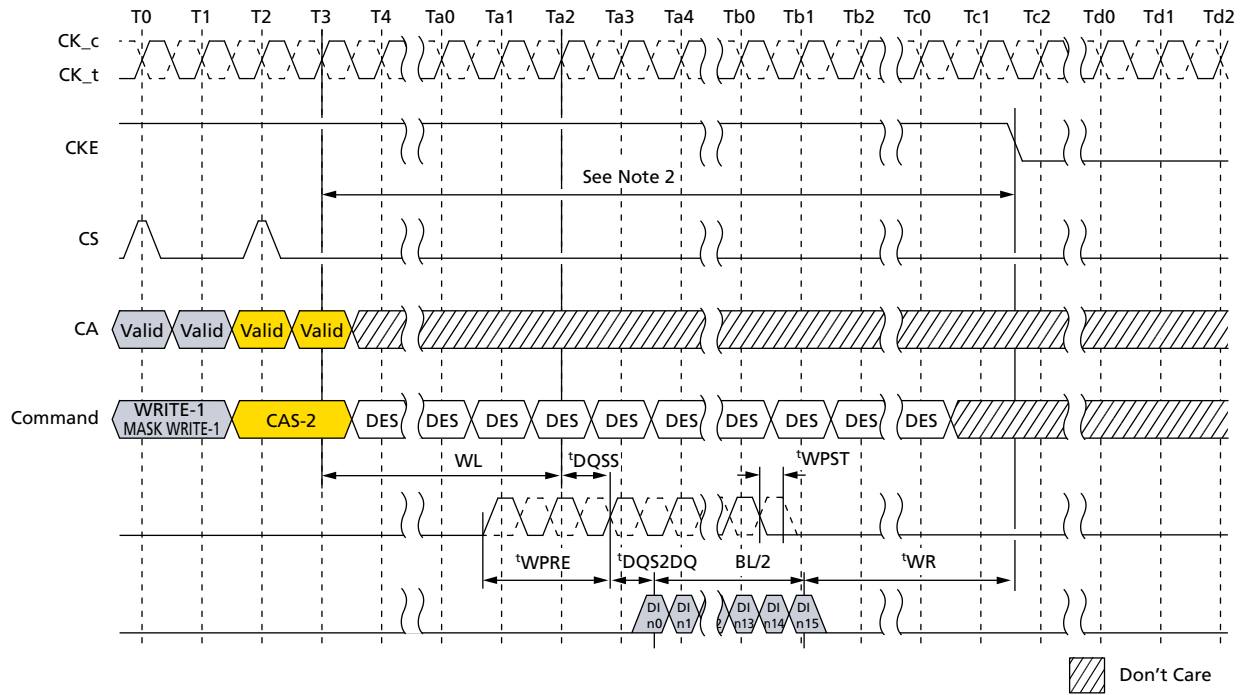
Figure 95: Write and Mask Write to Power-Down Entry
