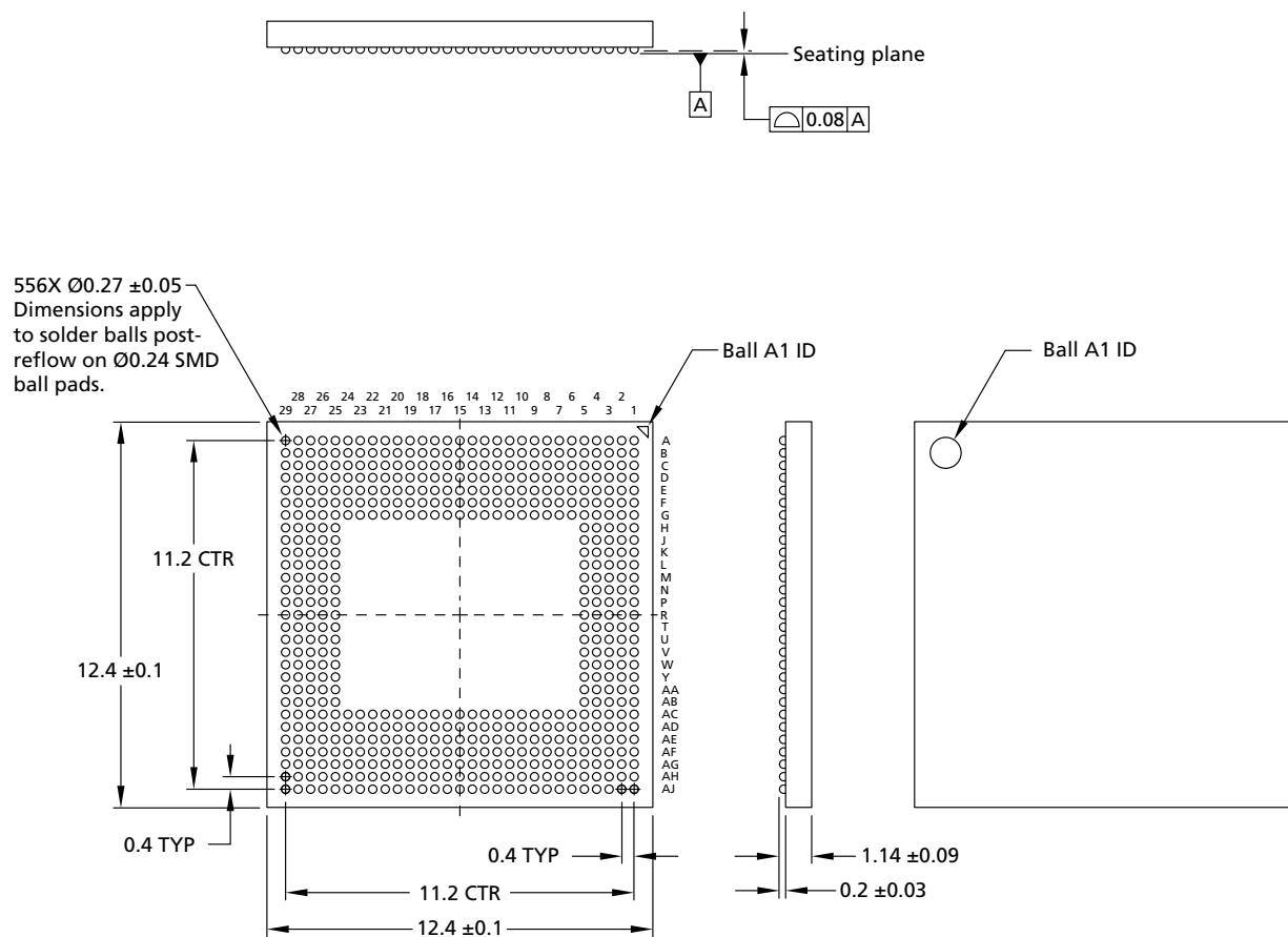
Figure 20: 556-Ball LFBGA – 12.4mm x 12.4mm x 1.23mm (Package Code: TN)
