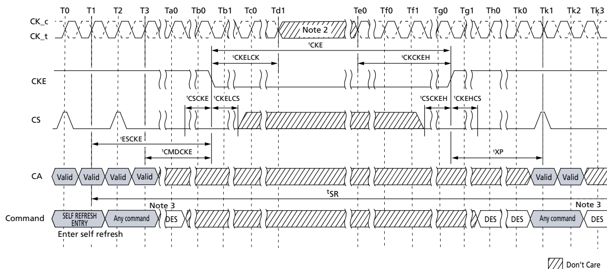
Figure 90: Command Input Timings after Power-Down Exit During Self Refresh
