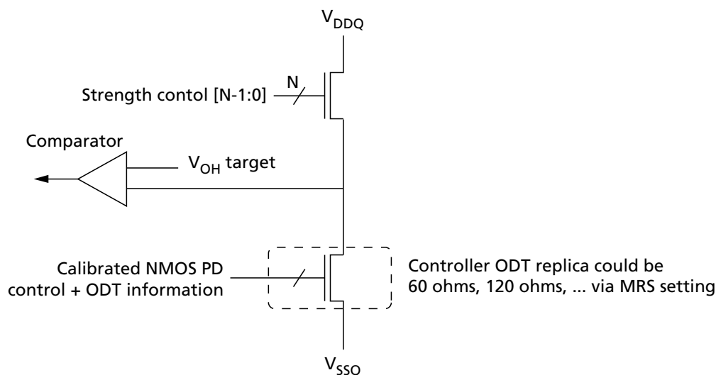
Figure 199: Pull-Up Calibration
