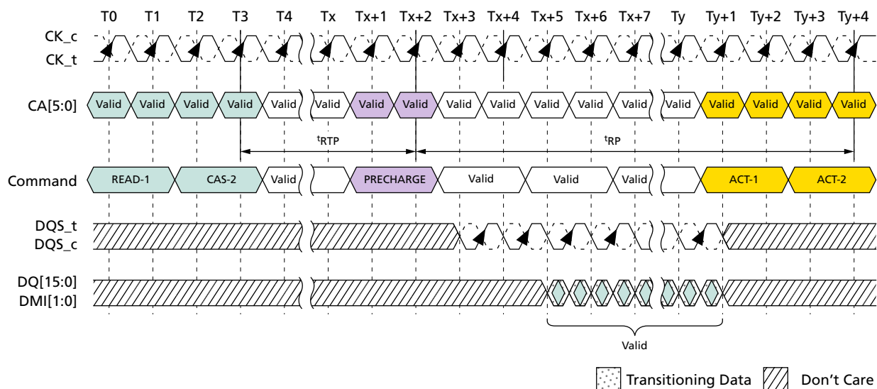
Figure 74: Burst READ Followed by Precharge – BL16, Toggling Preamble, 0.5nCK Postamble
