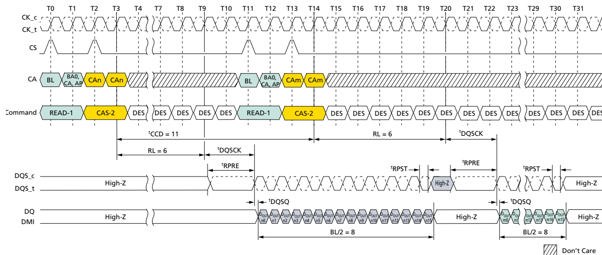
Figure 63: Consecutive READ: t_{CCD} = \text{MIN} + 3 , Preamble = Static, 0.5n\text{CK} Postamble
