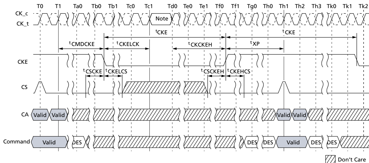
Figure 93: Basic Power-Down Entry and Exit Timing
