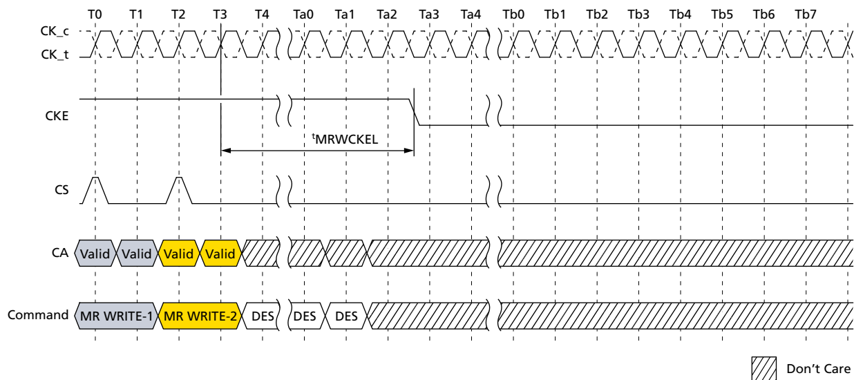
Figure 101: Mode Register Write to Power-Down Entry
