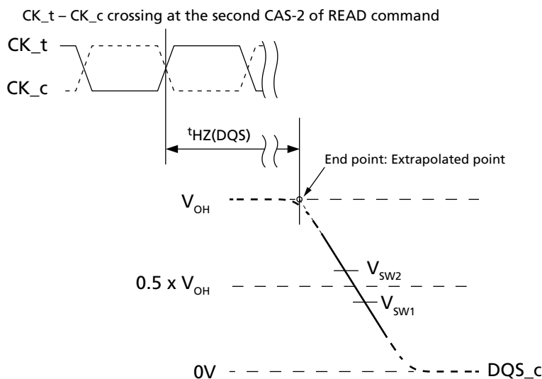
Figure 35: t_{HZ}(\text{DQS}) Method for Calculating Transitions and Endpoint
