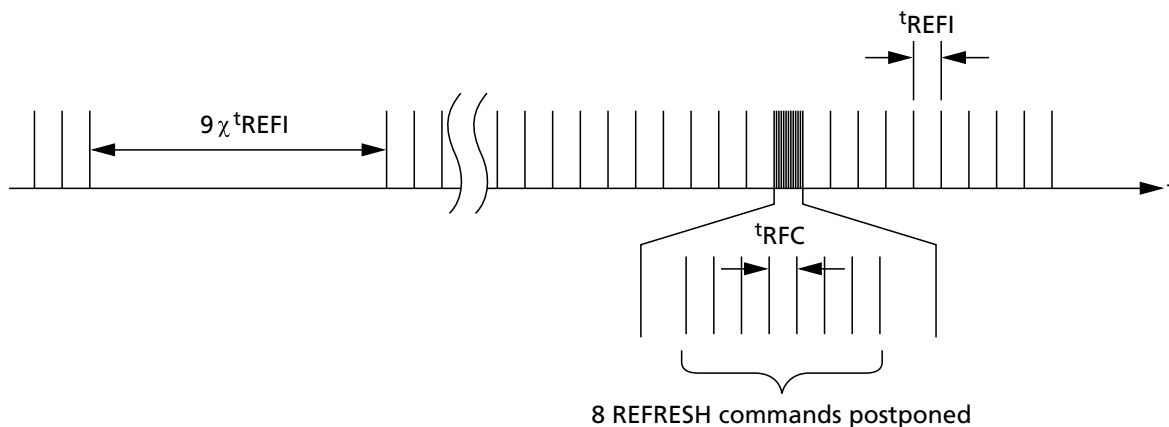
Figure 84: Postponing REFRESH Commands (Example)
