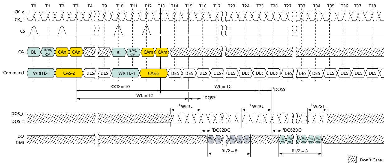
Figure 70: Consecutive WRITE: t_{\text{CCD}} = \text{MIN} + 2, 1.5n\text{CK} Postamble
