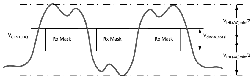
Figure 189: DQ V_{IHL(AC)} Definition (for Each Input Pulse)
