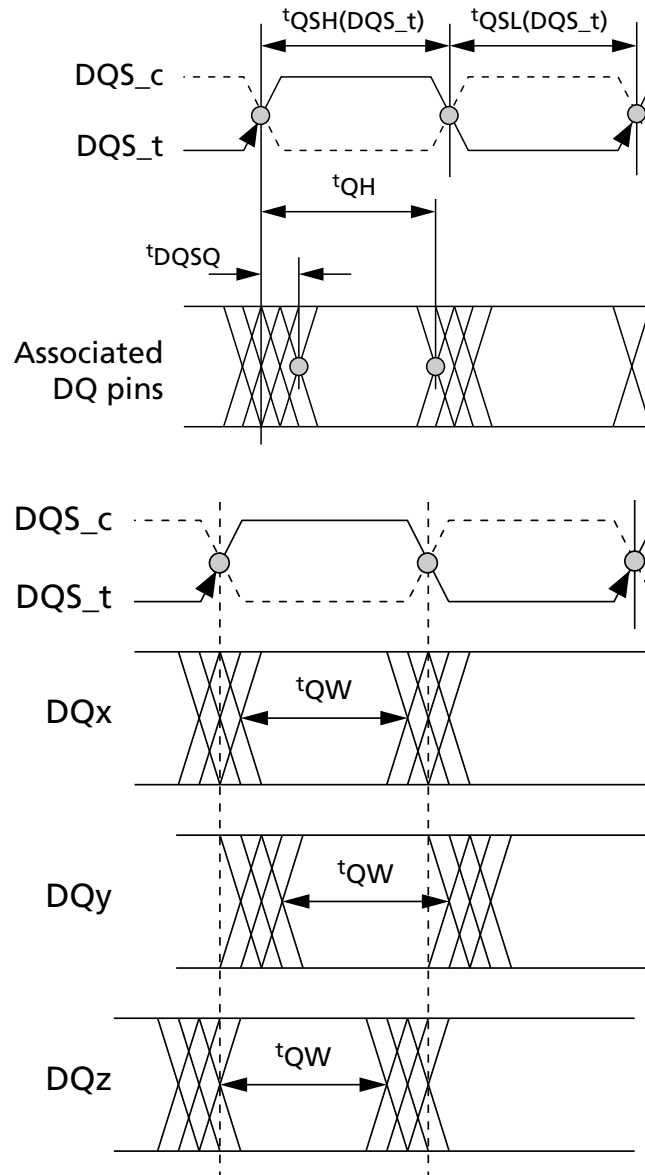
Figure 184: Read Data Timing Definitions – t_{QH} and t_{DQSQ} Across DQ Signals per DQS Group
