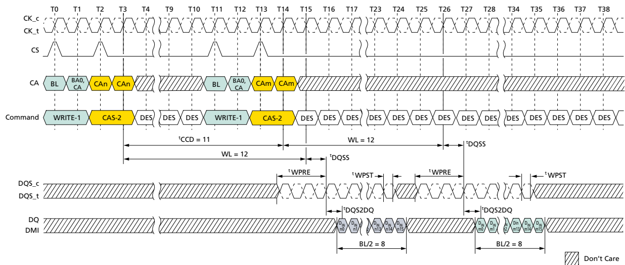
Figure 71: Consecutive WRITE: t_{CCD} = \text{MIN} + 3, 0.5n\text{CK} Postamble
