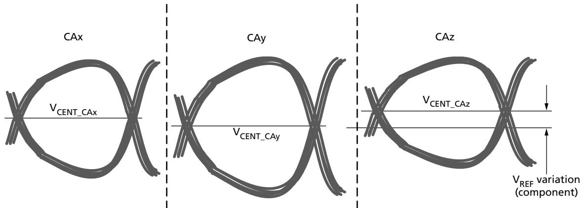
Figure 180: Across Pin V_{REF(CA)} Voltage Variation
