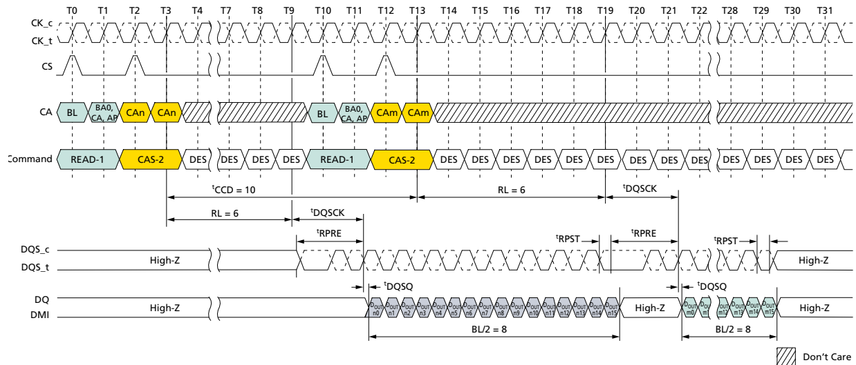
Figure 57: Consecutive READ: t_{CCD} = \text{MIN} + 2 , Preamble = Toggle, 0.5nCK Postamble
