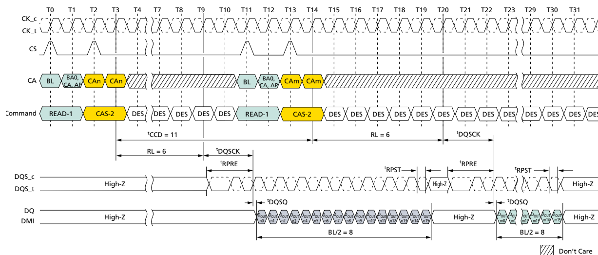
Figure 61: Consecutive READ: t_{CCD} = \text{MIN} + 3 , Preamble = Toggle, 0.5nCK Postamble
