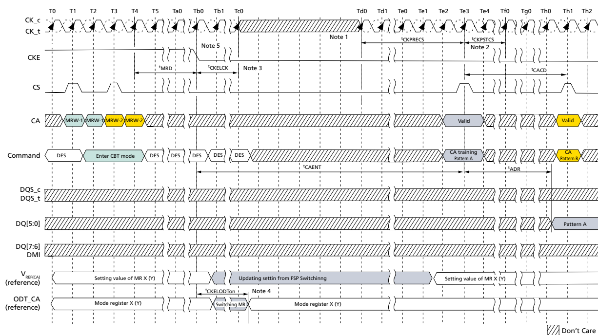
Figure 200: Entering CBT Mode and CA Training Pattern (Input and Output)
