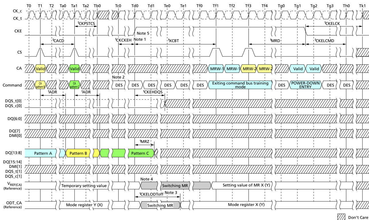
Figure 127: Command Bus Training Mode Exit with Power-Down Entry
