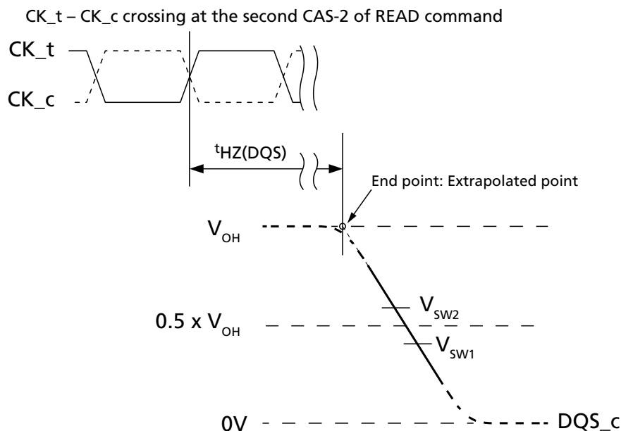
Figure 191: t_{HZ}(DQS) Method for Calculating Transitions and Endpoint
