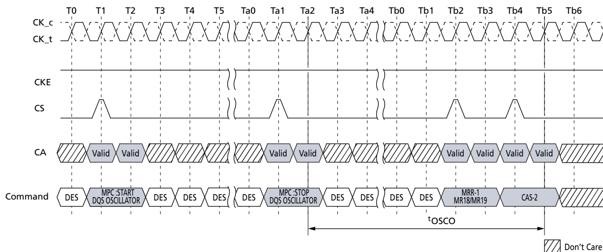
Figure 144: In Case of DQS Interval Oscillator is Stopped by MPC Command
