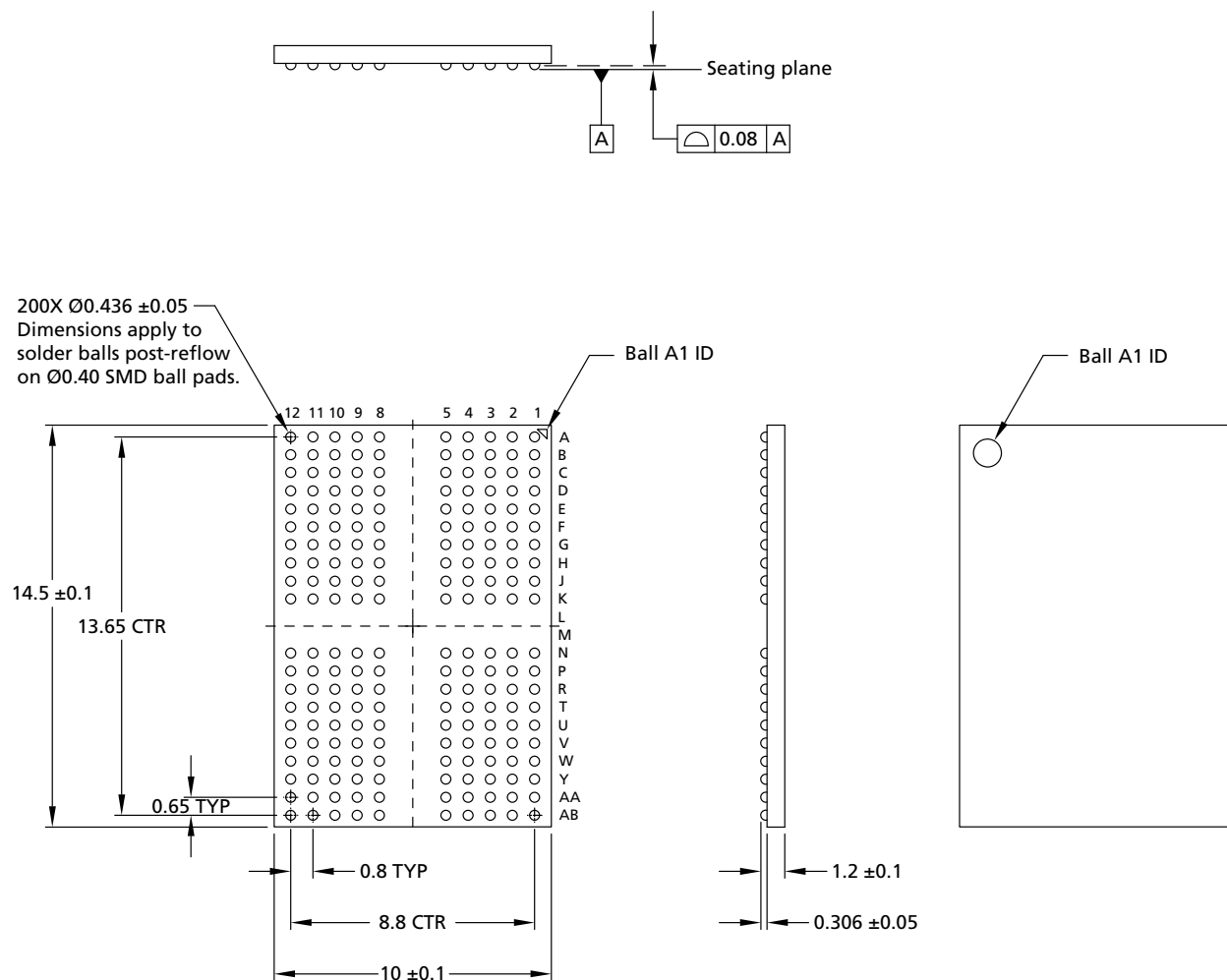
Figure 17: 200-Ball LFBGA – 10mm x 14.5mm x 1.3mm (Package Code: GS)
