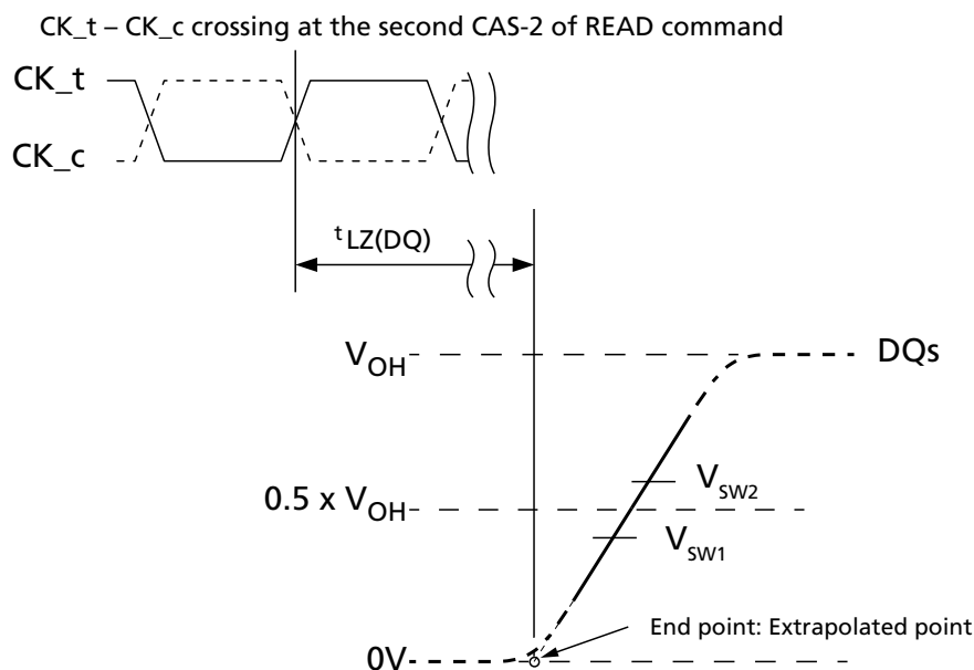
Figure 192: t_{LZ}(DQ) Method for Calculating Transitions and Endpoint
