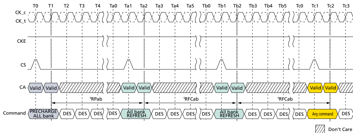
Figure 82: All-Bank REFRESH Operation
