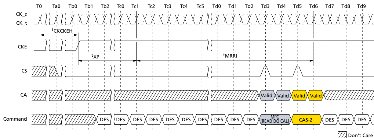
Figure 137: MPC[READ DQ CALIBRATION] Following Power-Down State
