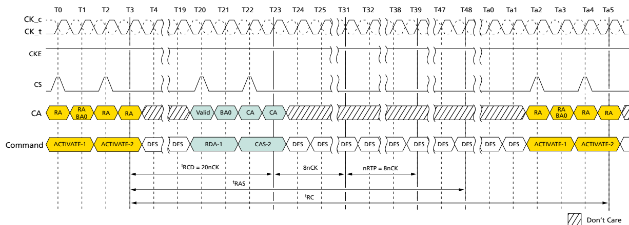
Figure 80: Command Input Timing with RAS Lock
