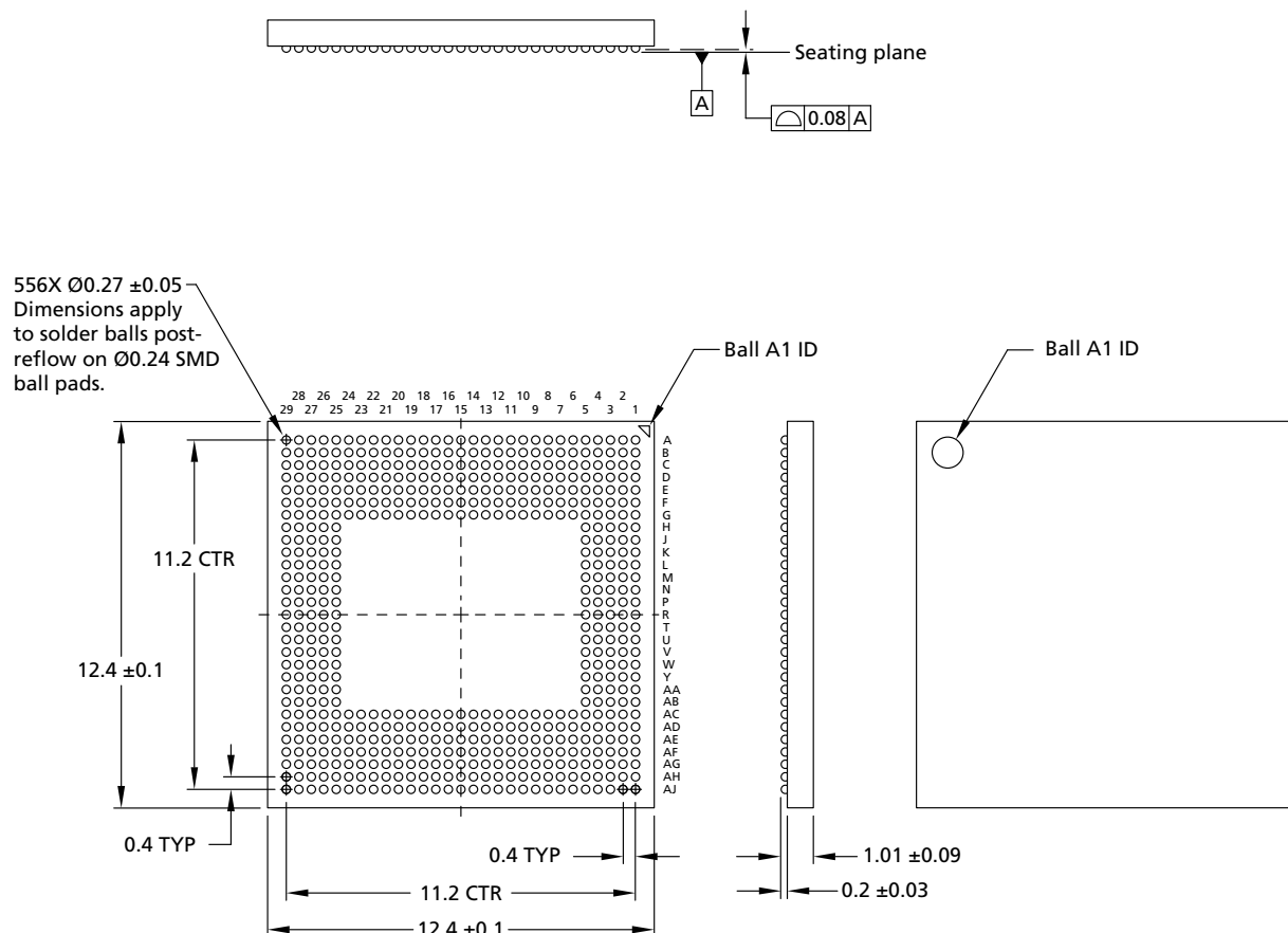
Figure 19: 556-Ball TFBGA – 12.4mm x 12.4mm x 1.1mm (Package Code: HJ)
