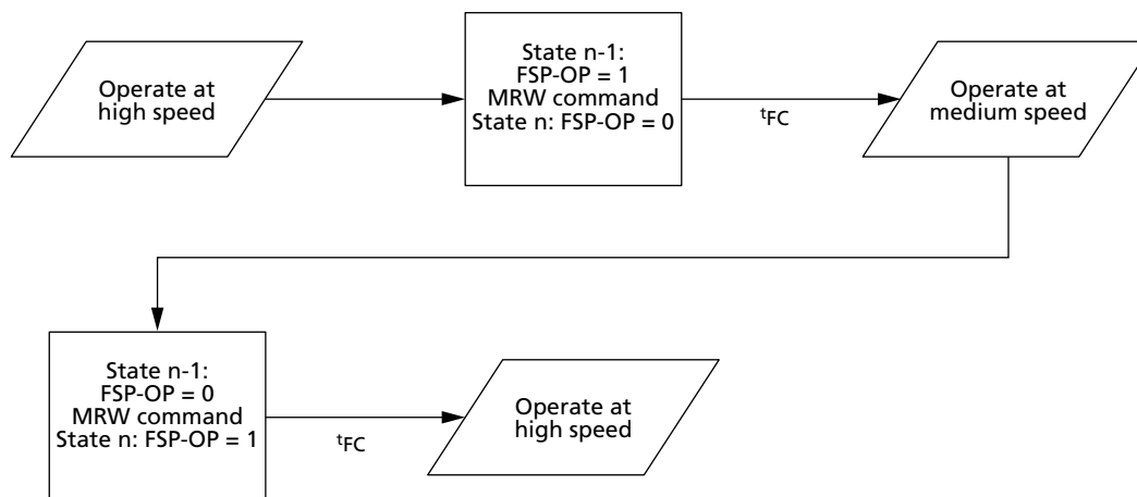
Figure 150: Example of Switching Between Two Trained Frequency Set Points
