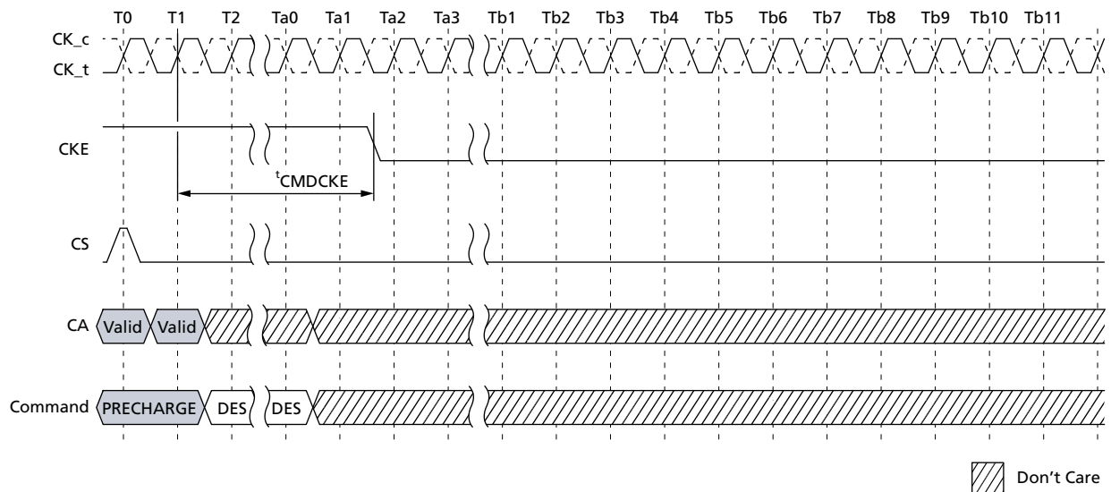
Figure 99: PRECHARGE Command to Power-Down Entry
