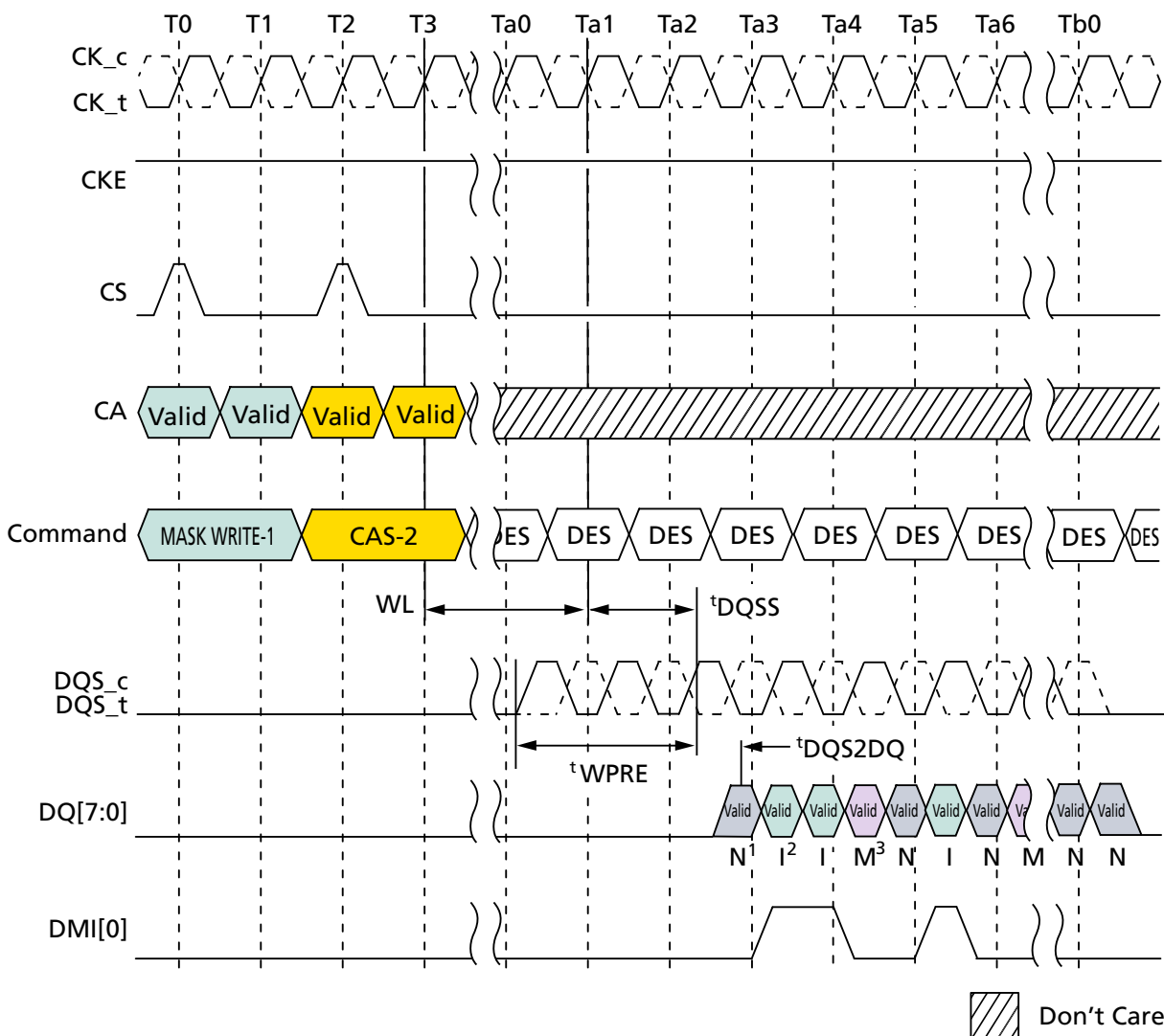
Figure 45: MASKED WRITE Command with Write DBI Enabled; DM Enabled
