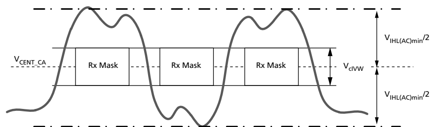
Figure 183: CA V_{IHL\_AC} Definition (for Each Input Pulse)
