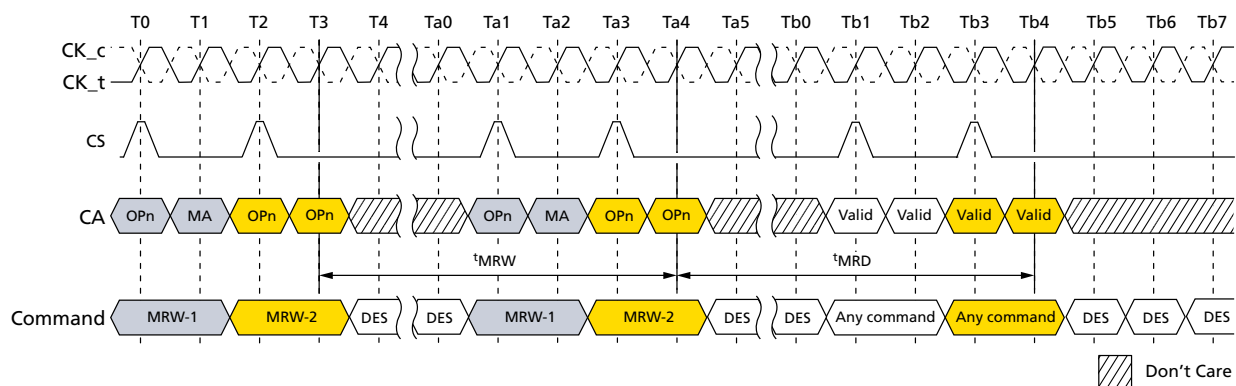
Figure 107: MODE REGISTER WRITE Timing
