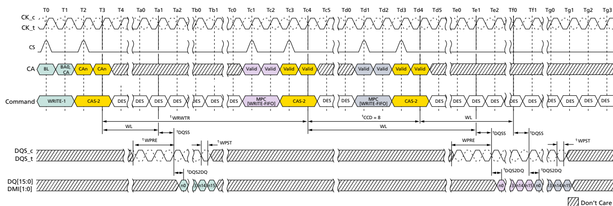
Figure 138: WRITE-to-MPC[WRITE-FIFO] Operation Timing
