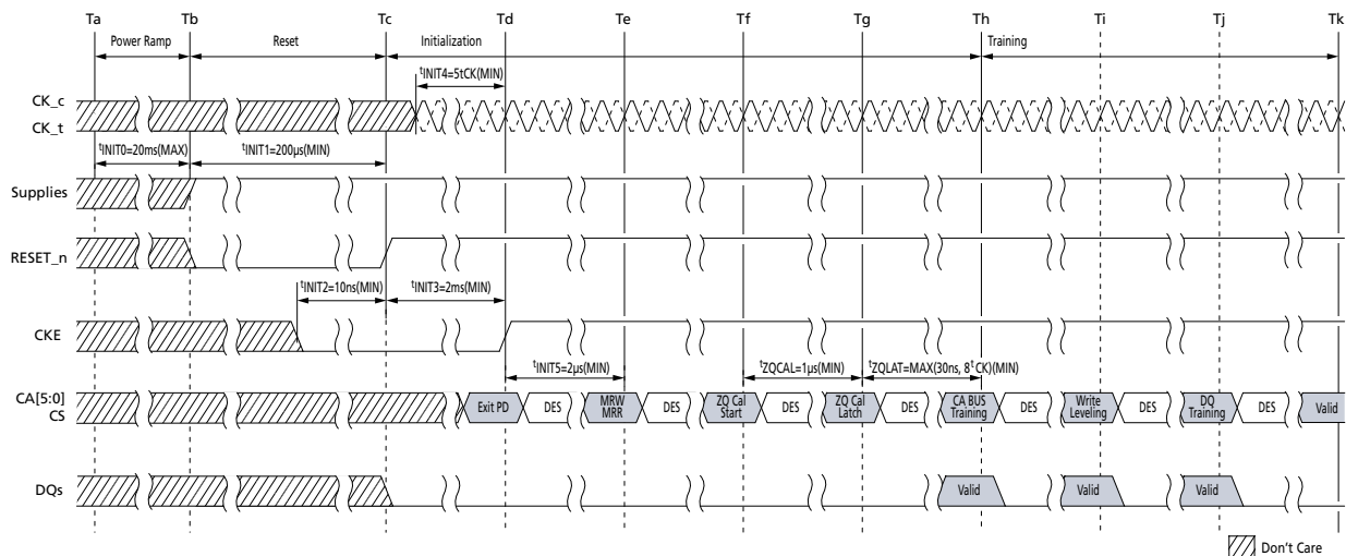
Figure 23: Voltage Ramp and Initialization Sequence
