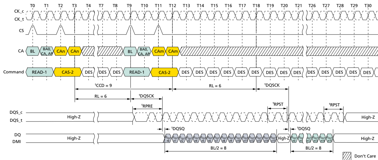
Figure 52: Seamless READ: t_{CCD} = \text{MIN} + 1 , Preamble = Toggle, 1.5nCK Postamble
