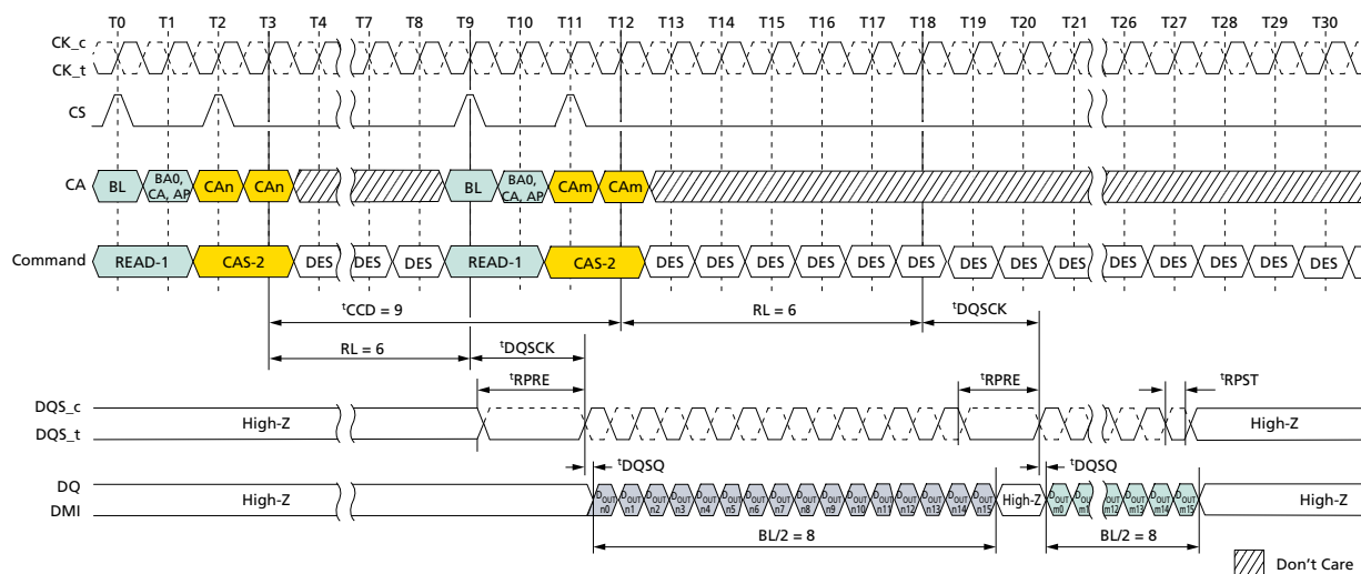
Figure 55: Consecutive READ: t_{CCD} = \text{MIN} + 1 , Preamble = Static, 0.5n\text{CK} Postamble
