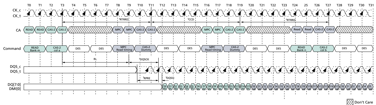
Figure 208: Read DQ Calibration Training Timing
