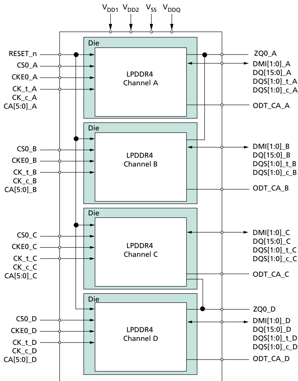
Figure 6: Quad-Die, Quad-Channel, Single-Rank Package Block Diagram
