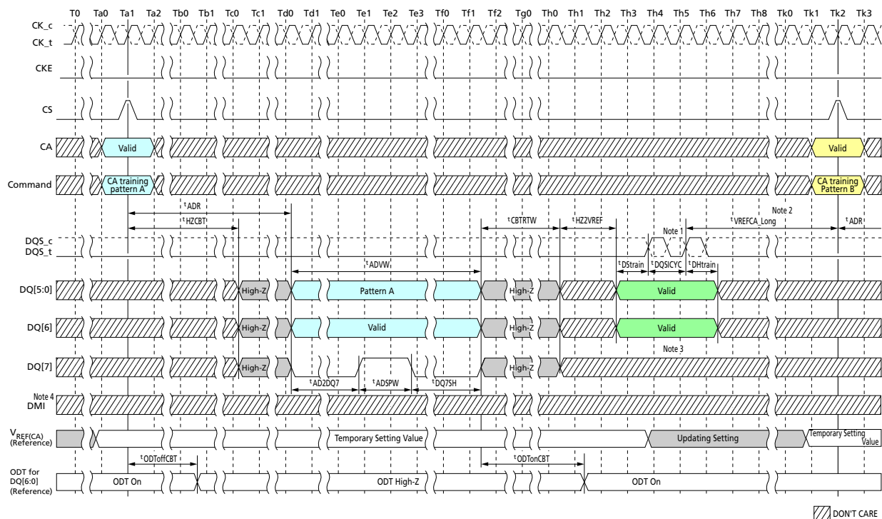
Figure 204: CA Pattern Input/Output to V_{REF} Setting Input
