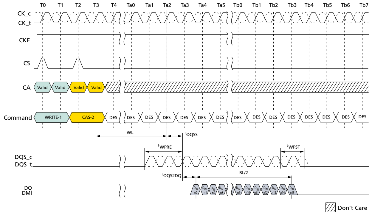
Figure 29: DQS Write Preamble and Postamble – 1.5nCK Postamble
