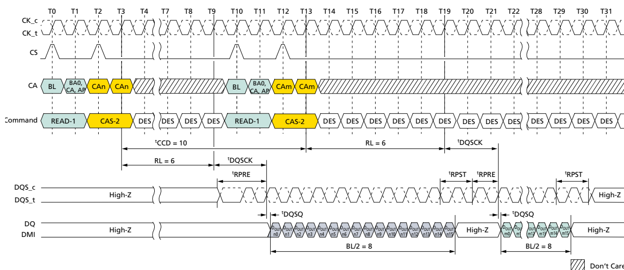
Figure 56: Consecutive READ: t_{CCD} = \text{MIN} + 2 , Preamble = Toggle, 1.5n\text{CK} Postamble
