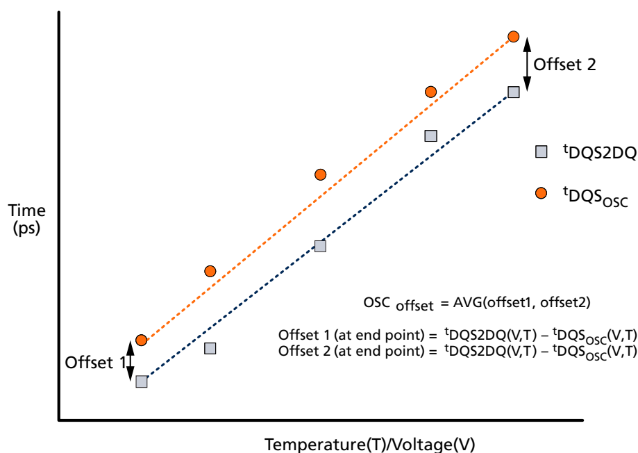
Figure 143: Interval Oscillator Offset – \text{OSC}_{\text{Offset}}
