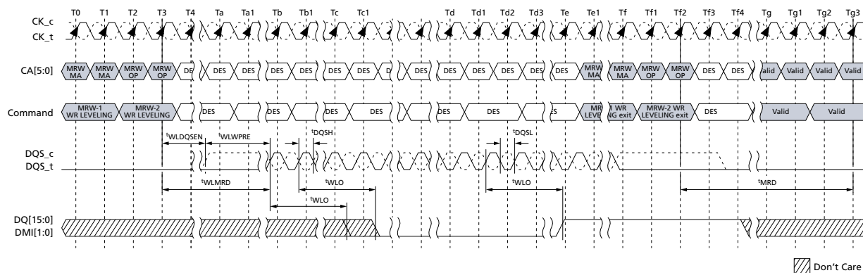
Figure 129: Write Leveling Timing – t_{DQSL}(\text{MIN})
