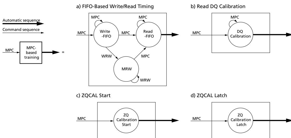
Figure 22: Simplified State Diagram
