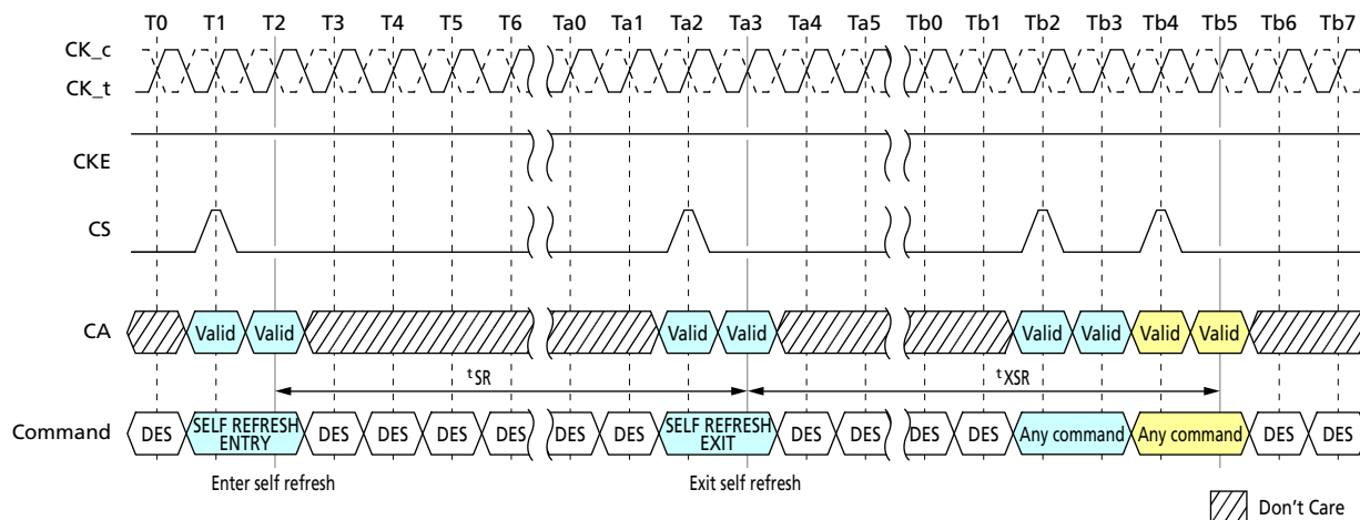
Figure 88: Self Refresh Entry/Exit Timing
