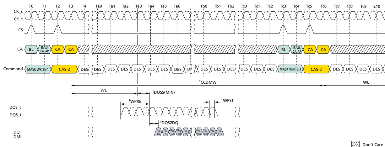
Figure 43: MASK WRITE Command – Same Bank
