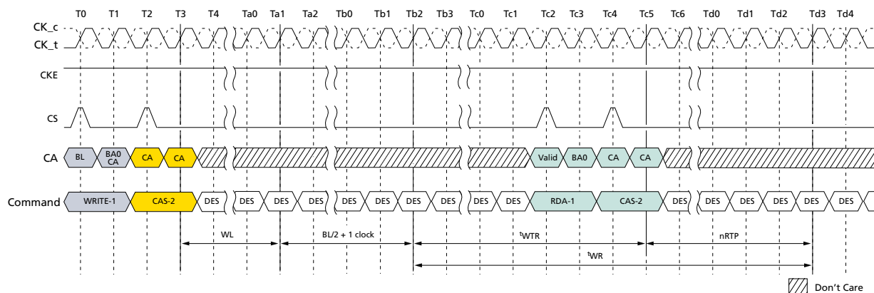
Figure 81: Delay Time From WRITE-to-READ with Auto Precharge
