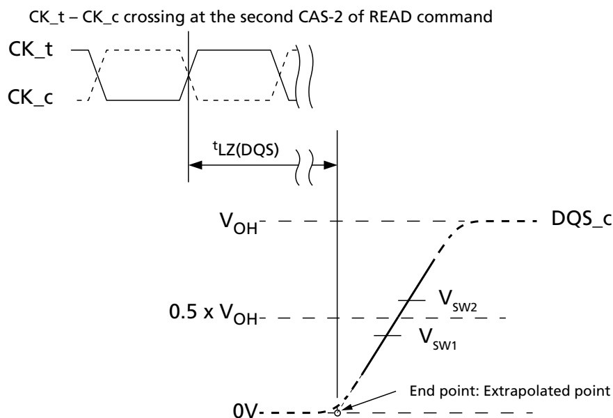
Figure 190: t_{LZ}(DQS) Method for Calculating Transitions and Endpoint
