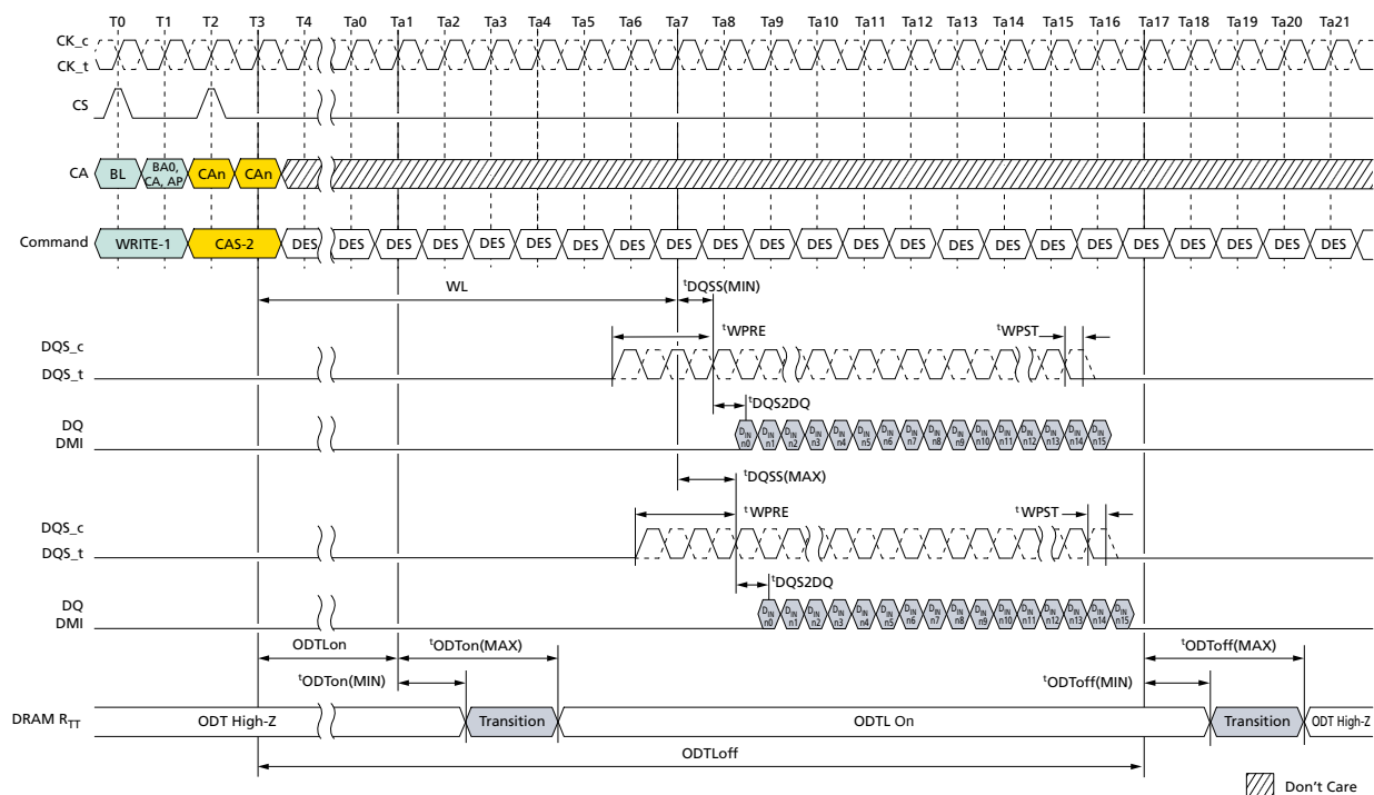
Figure 155: Asynchronous ODTon/ODToff Timing
