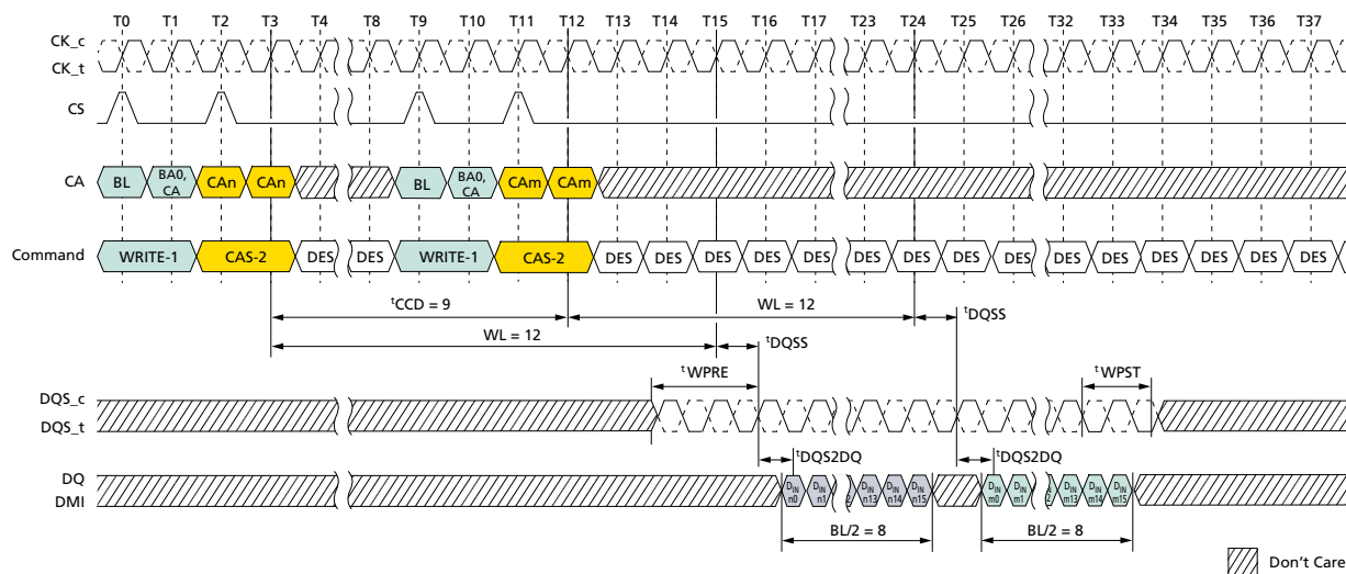
Figure 68: Consecutive WRITE: t_{CCD} = MIN + 1, 1.5nCK Postamble
