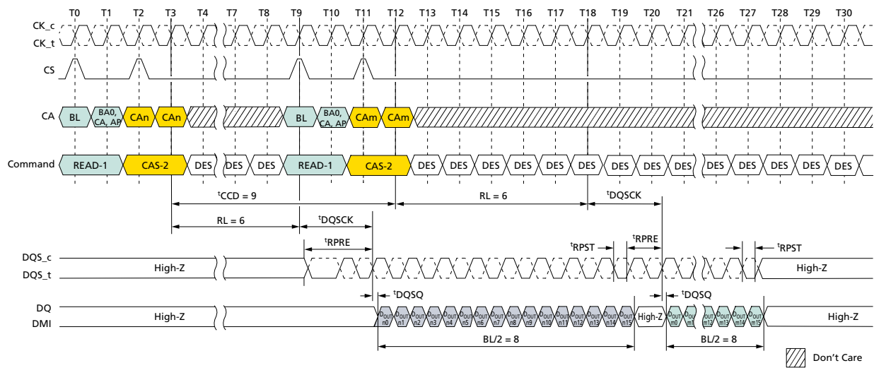
Figure 53: Consecutive READ: t_{CCD} = \text{MIN} + 1 , Preamble = Toggle, 0.5n\text{CK} Postamble
