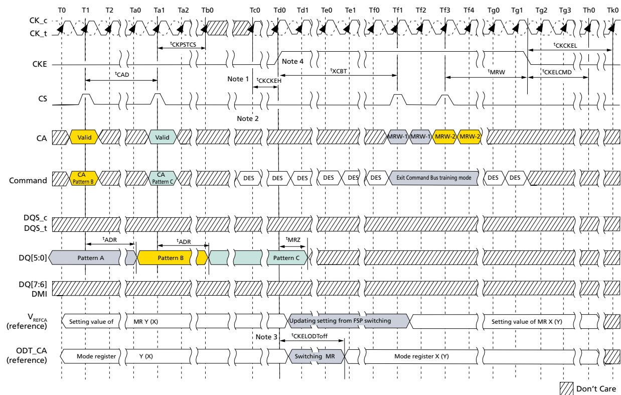
Figure 202: Exiting CBT Mode with Power Down Entry
