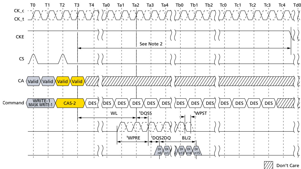
Figure 96: Write With Auto Precharge and Mask Write With Auto Precharge to Power-Down Entry
