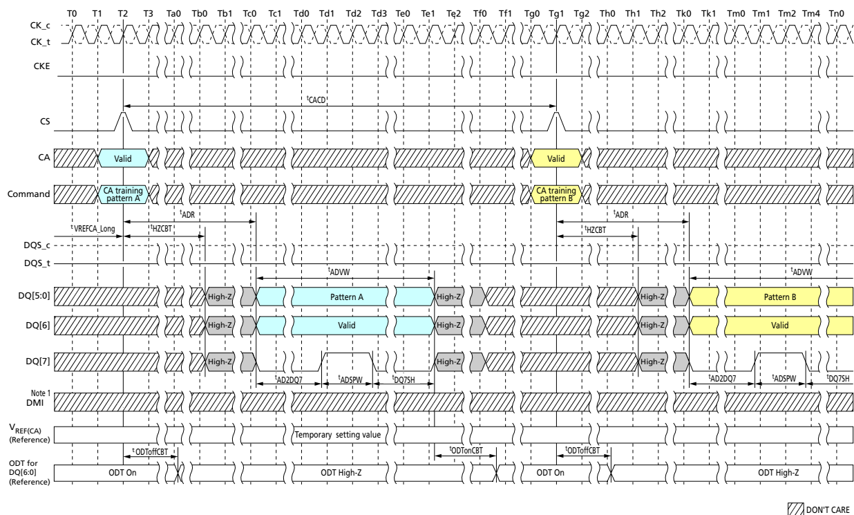
Figure 205: Consecutive CA Training Pattern Input/Output
