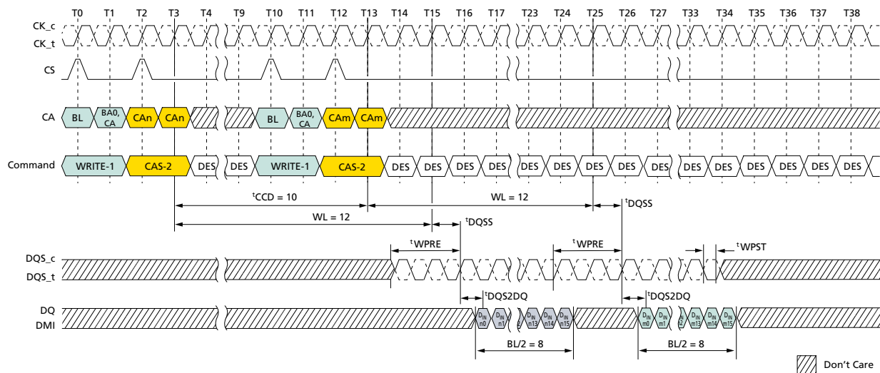
Figure 69: Consecutive WRITE: t_{CCD} = MIN + 2, 0.5nCK Postamble
