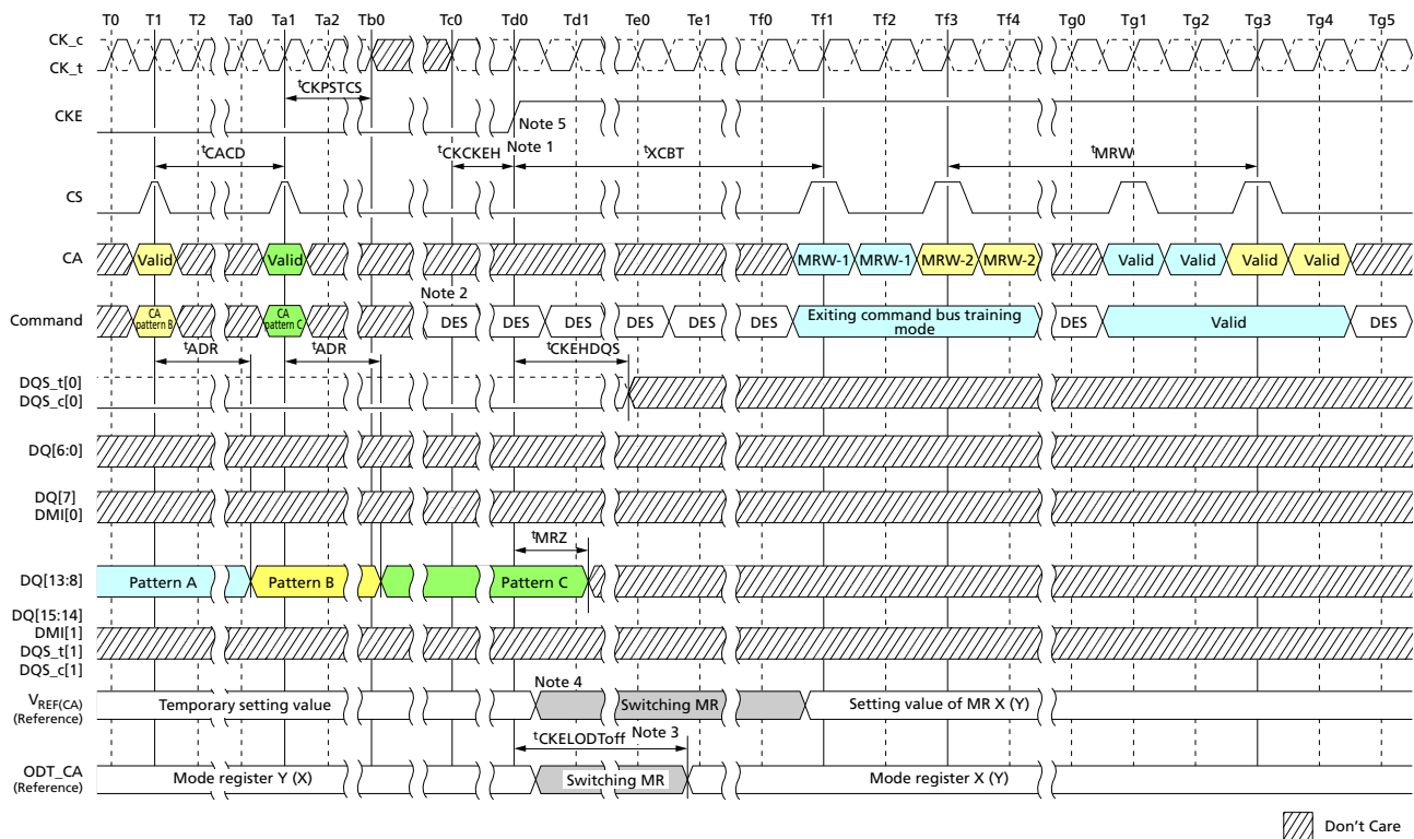
Figure 126: Command Bus Training Mode Exit with Valid Command
