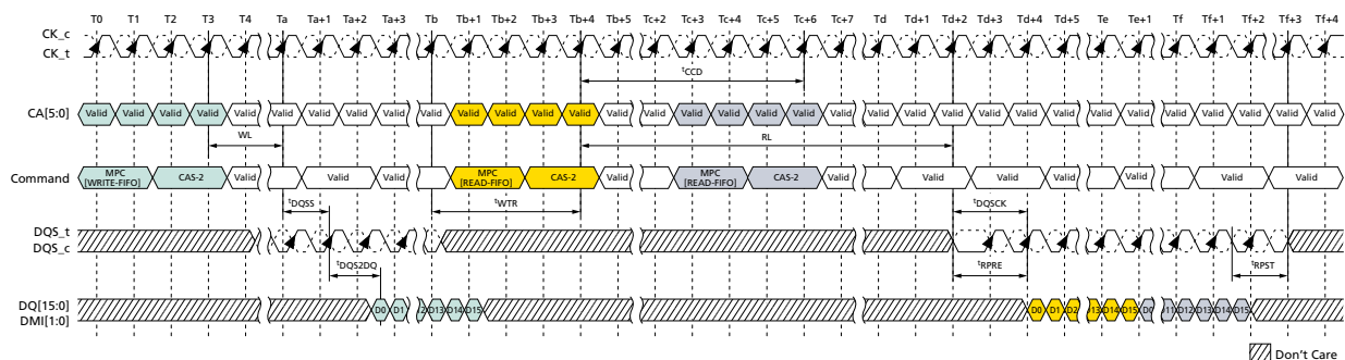
Figure 133: READ-FIFO – t_{WPRE} = 2nCK , t_{WPST} = 0.5nCK , t_{RPRE} = \text{Toggle} , t_{RPST} = 1.5nCK
