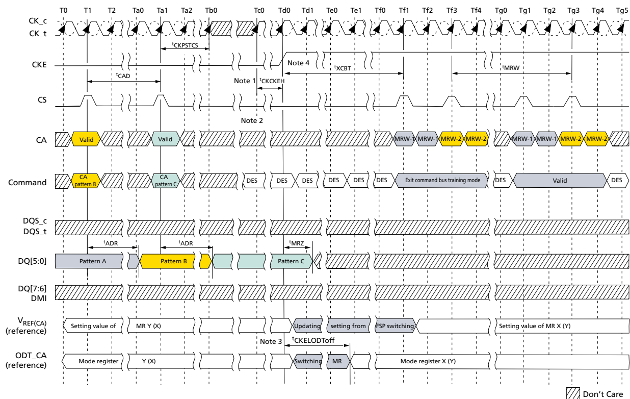
Figure 201: Exiting CBT Mode with Valid Command
