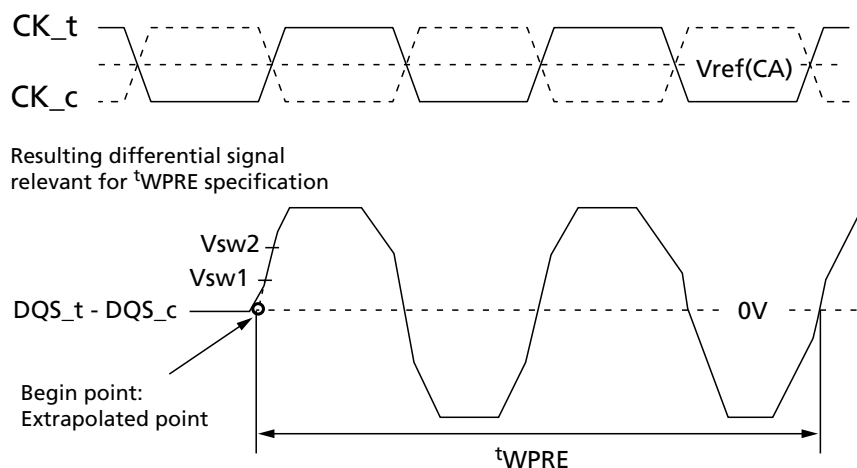
Figure 41: Method for Calculating t WPRE Transitions and Endpoints
