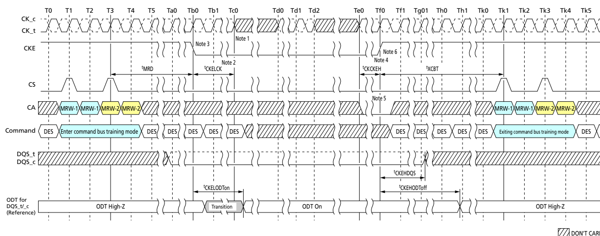
Figure 207: DQS ODT Timing during Command Bus Training Mode 2
