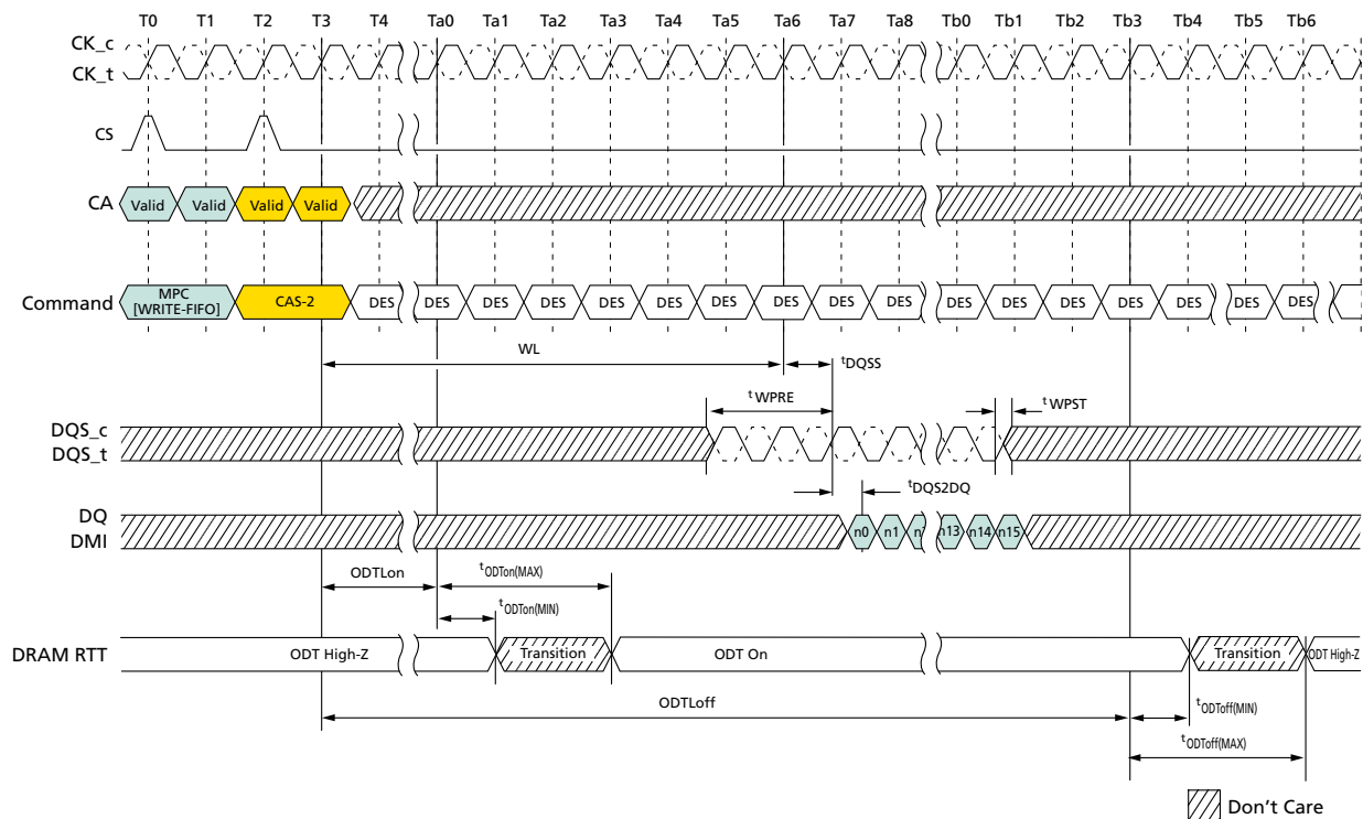
Figure 141: MPC[WRITE-FIFO] with DQ ODT Timing
