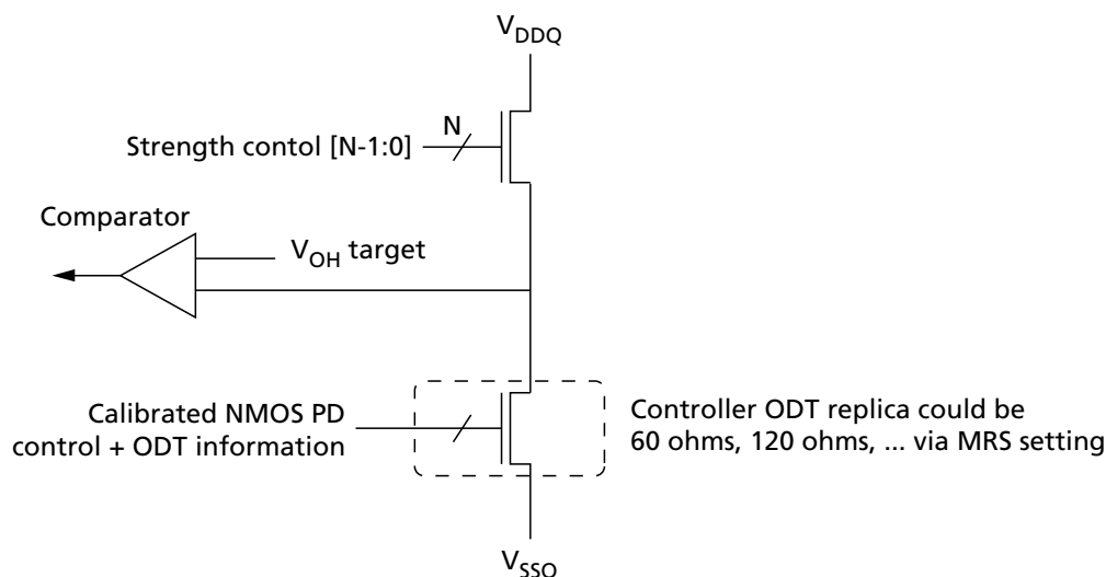
Figure 176: Pull-Up Calibration
