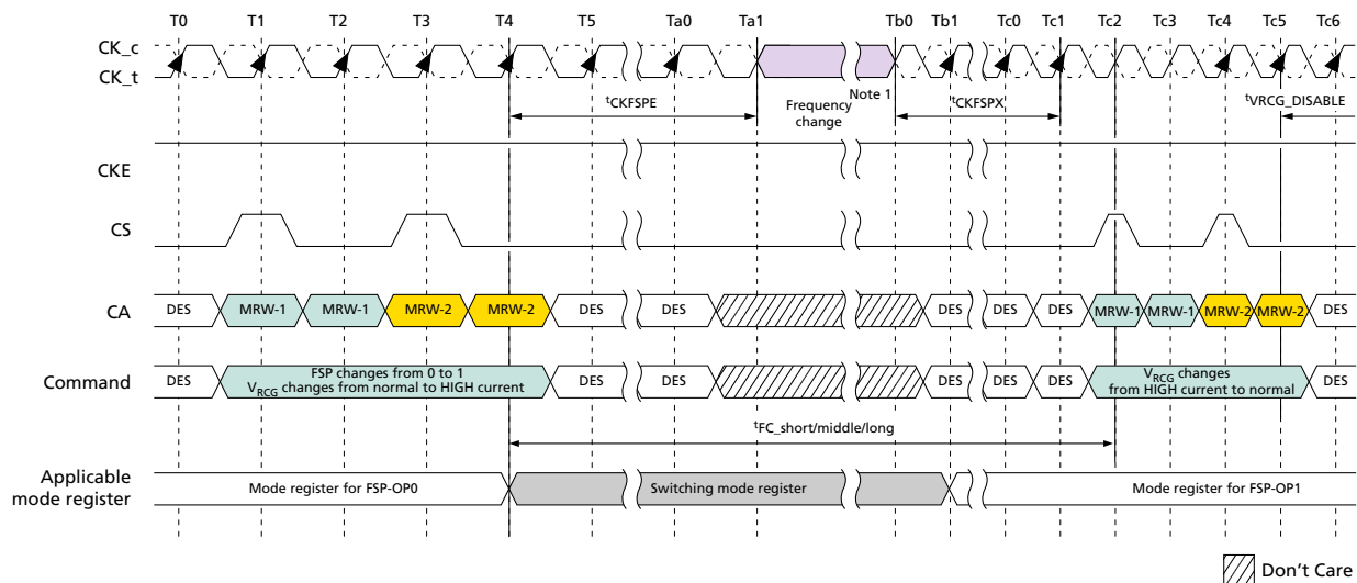
Figure 148: Frequency Set Point Switching Timing
