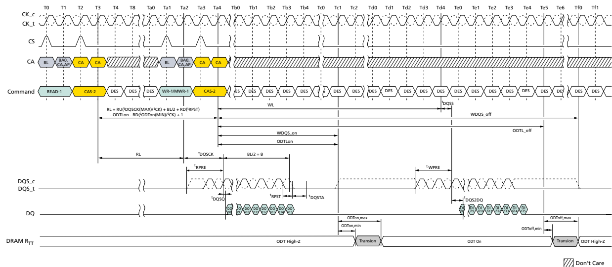
Figure 50: Burst READ Followed by Burst WRITE or Burst MASKED WRITE (ODT Enable)
