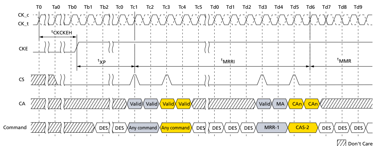
Figure 106: MRR Following Power-Down
