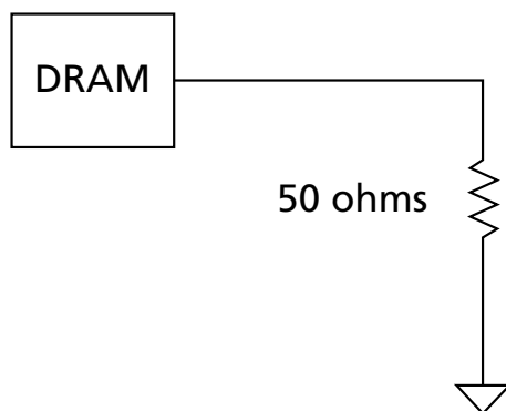
Figure 174: Driver Output Timing Reference Load
