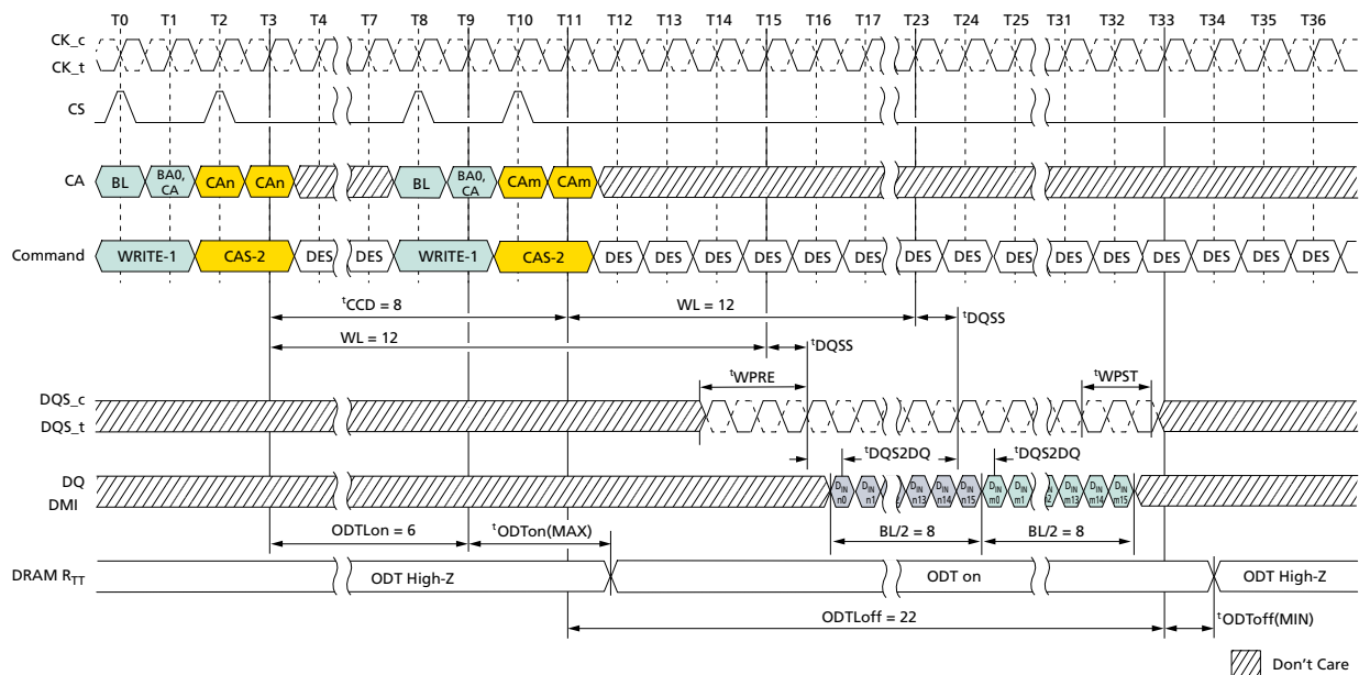
Figure 65: Seamless WRITE: t_{CCD} = \text{MIN} , 1.5nCK Postamble, 533 \text{ MHz} < \text{Clock Frequency} \leq 800 \text{ MHz} , ODT Worst Timing Case
