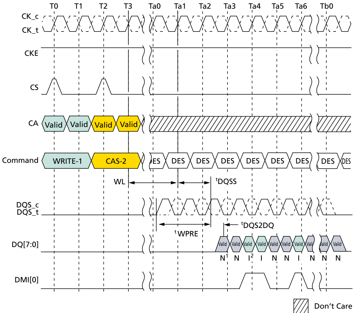
Figure 46: WRITE Command with Write DBI Enabled; DM Disabled
