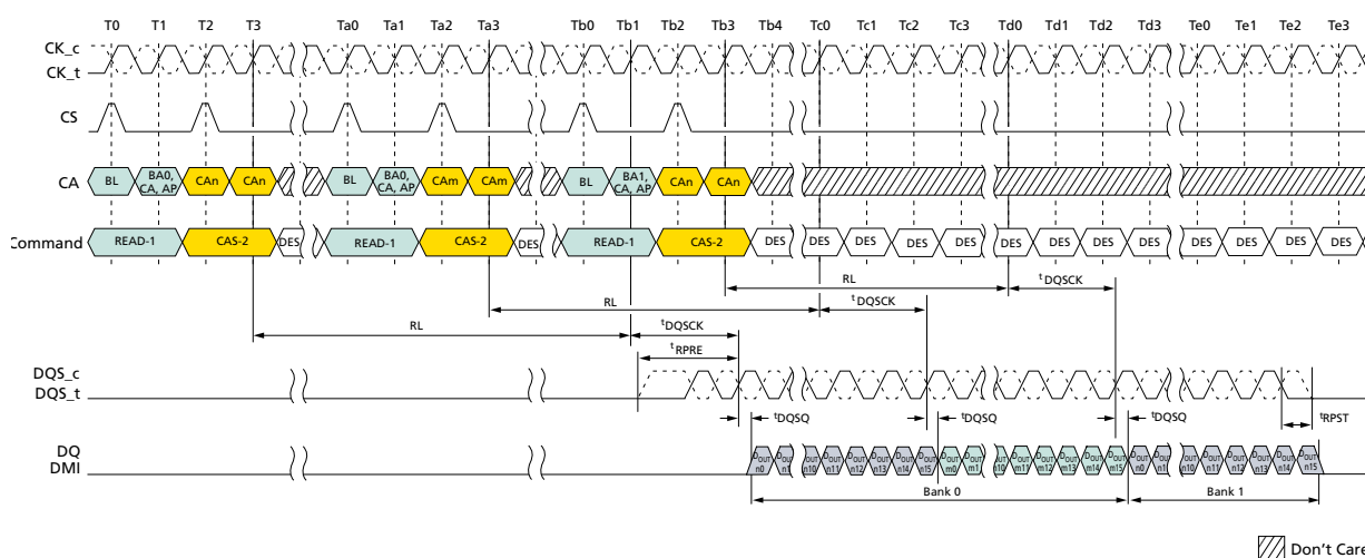
Figure 32: Seamless Burst Read
