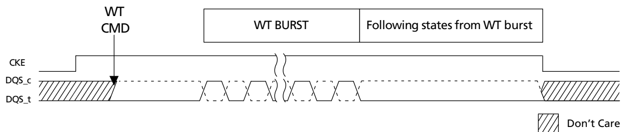
Figure 47: WDQS Control Mode 1
