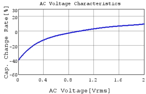
GRM185R61E105KA12 C-AC Voltage capchange, Dc
