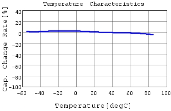
GRM185R61E105KA12 C-Temp. capchange, DC0.0V,
