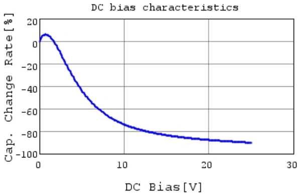
GRM185R61E105KA12 C-DC bias capchange, 25.0c
