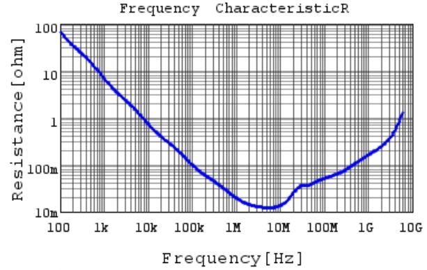
GRM185R61E105KA12 R DCOV, 25degC
