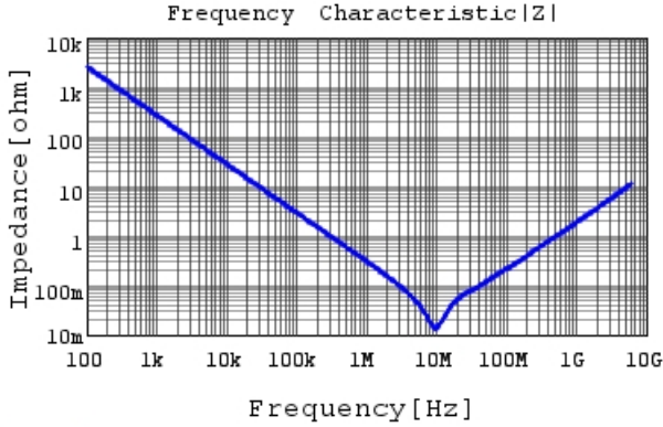
GRM185R61E105KA12 |Z| DCOV, 25degC
