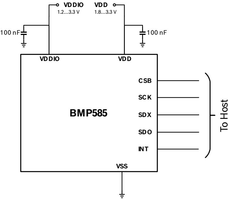
Figure 24: SPI 4-wire connection diagram
