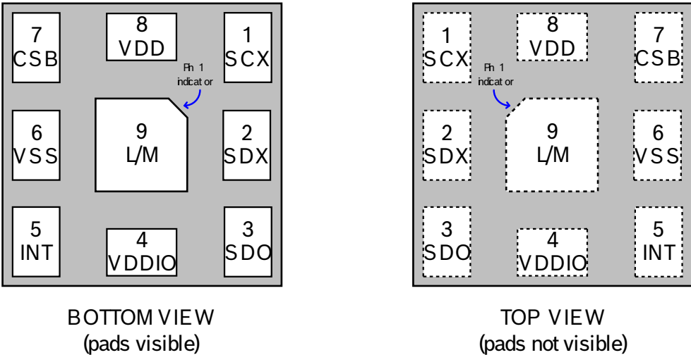
Figure 22: Pin out bottom and top view
