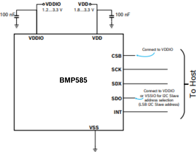
Figure 25: I²C connection diagram
