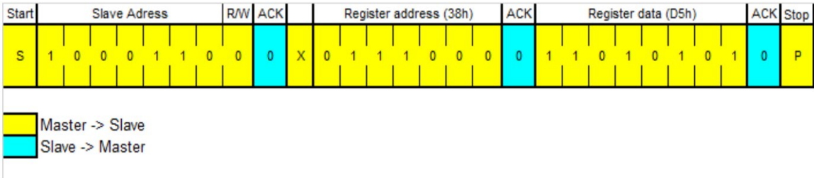
Figure 13: single-byte I 2 C write
