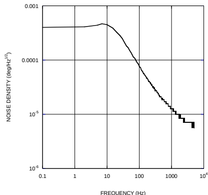
Noise Spectrum at 50mT and \tau = 16\text{ms}
