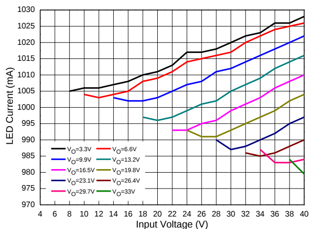
LED Current vs. Input Voltage ( R_S=0.1\Omega , L=68\mu\text{H} )
