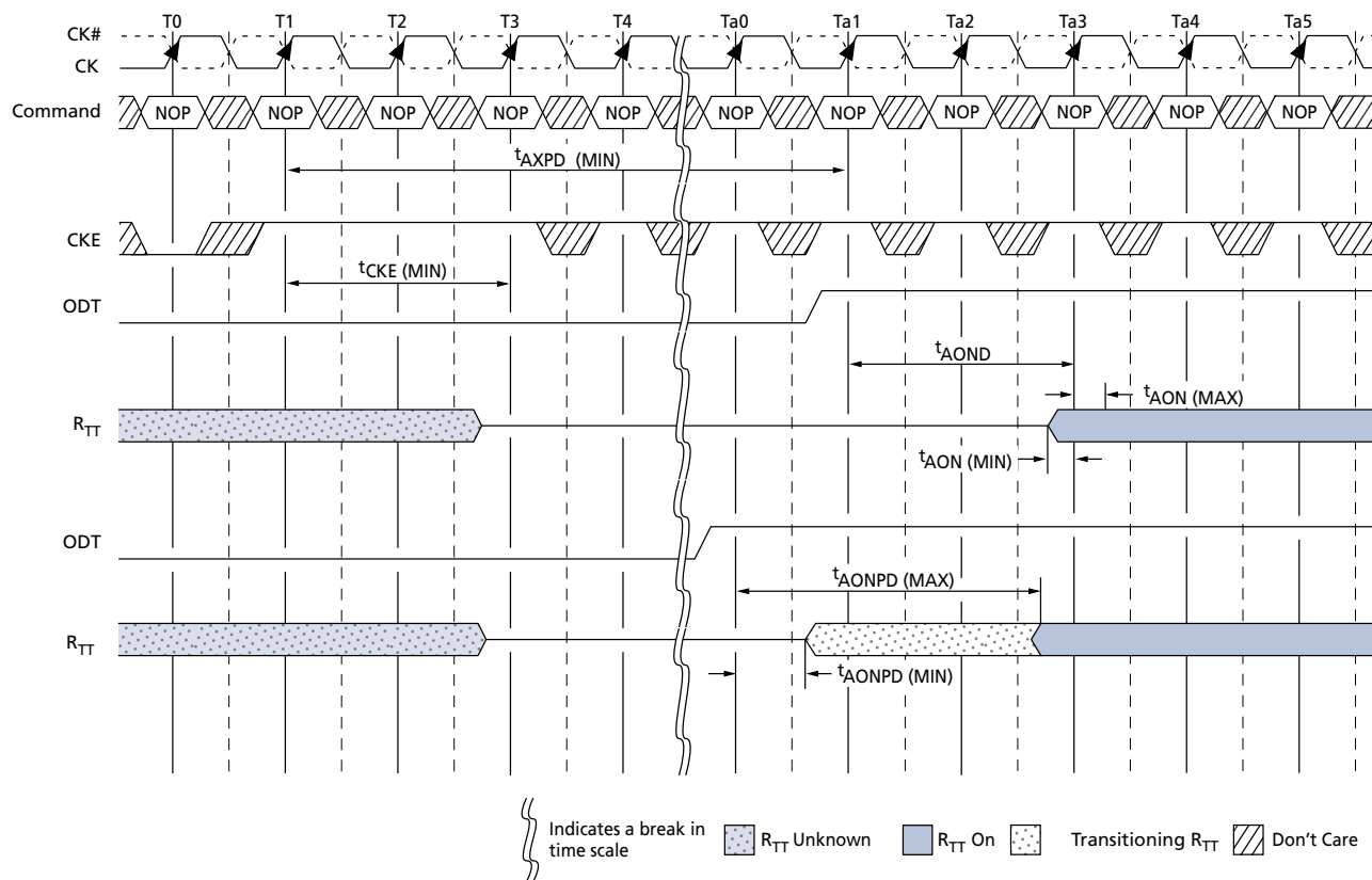
Figure 85: ODT Turn-On Timing When Exiting Power-Down Mode
