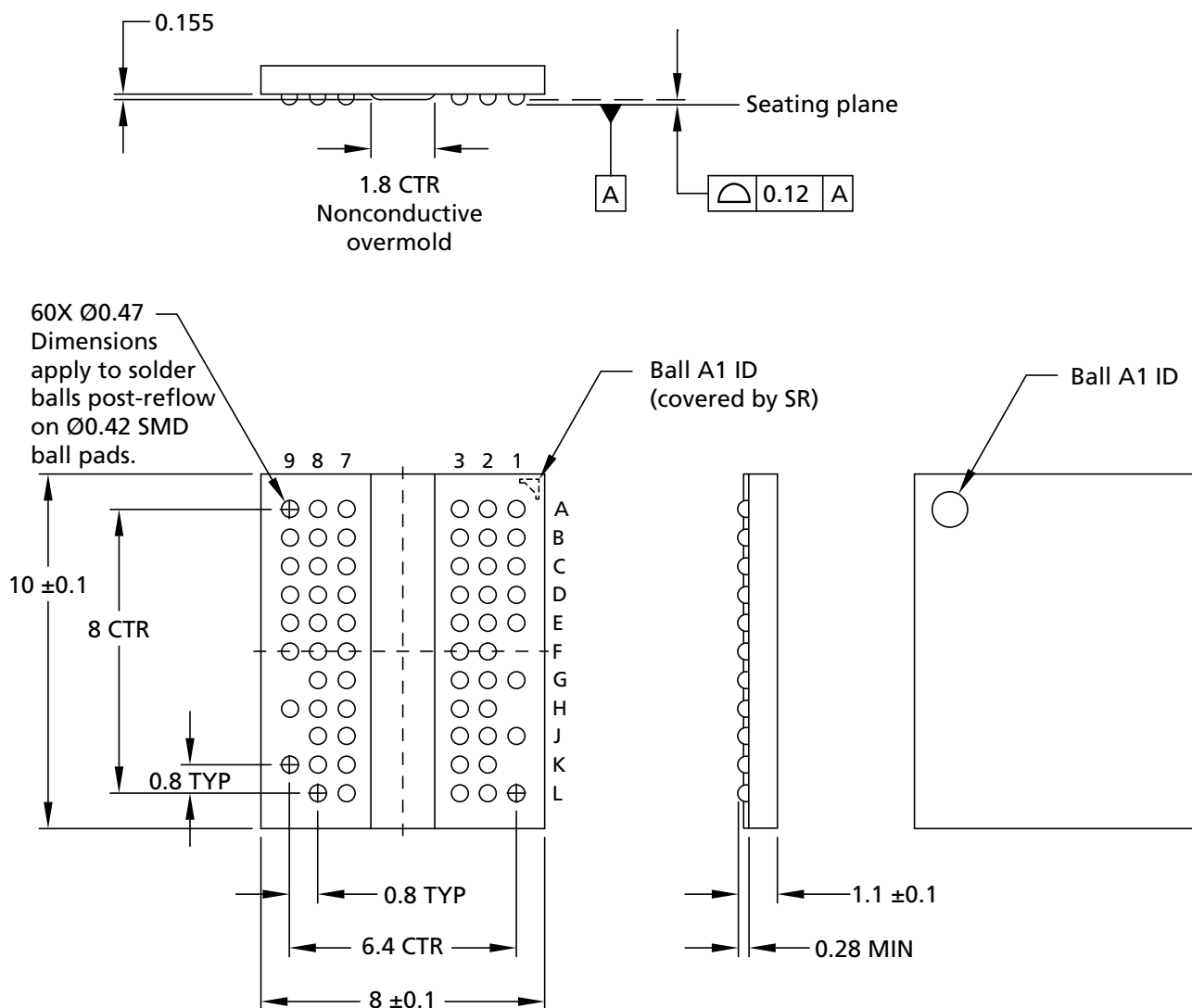
Figure 8: 60-Ball FBGA (8mm x 10mm) – x8; "SH" Die Rev :M
