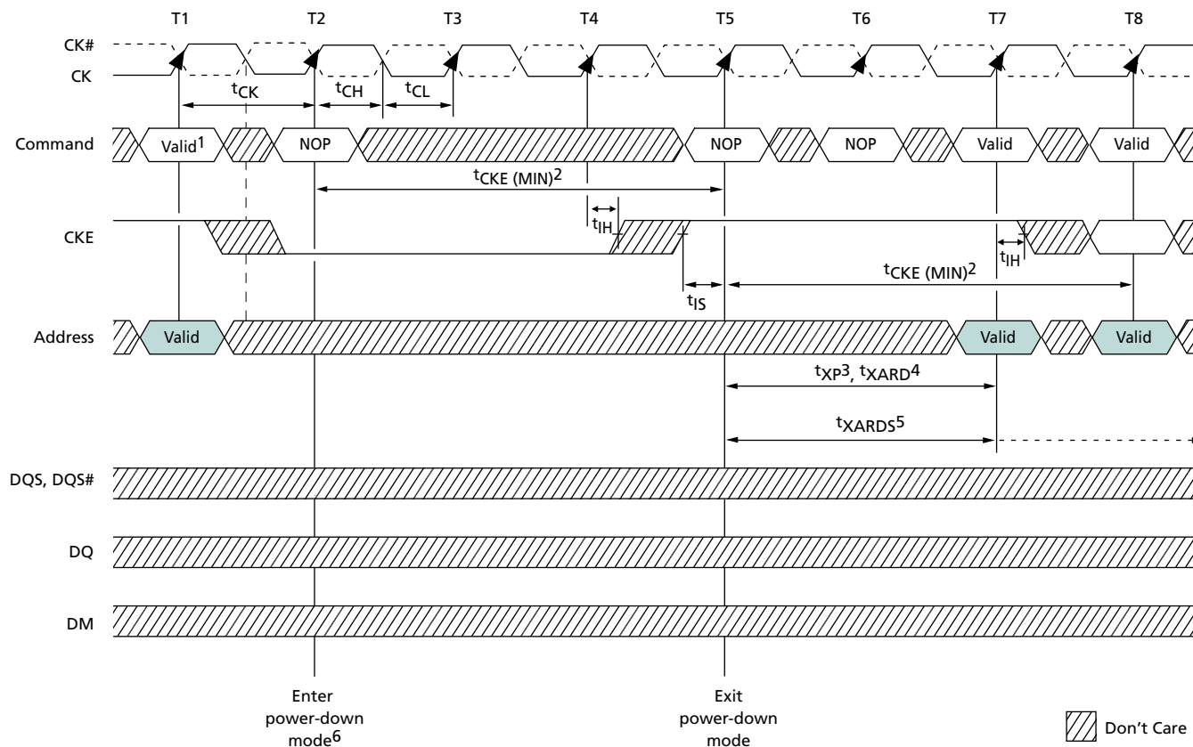
Figure 67: Power-Down
