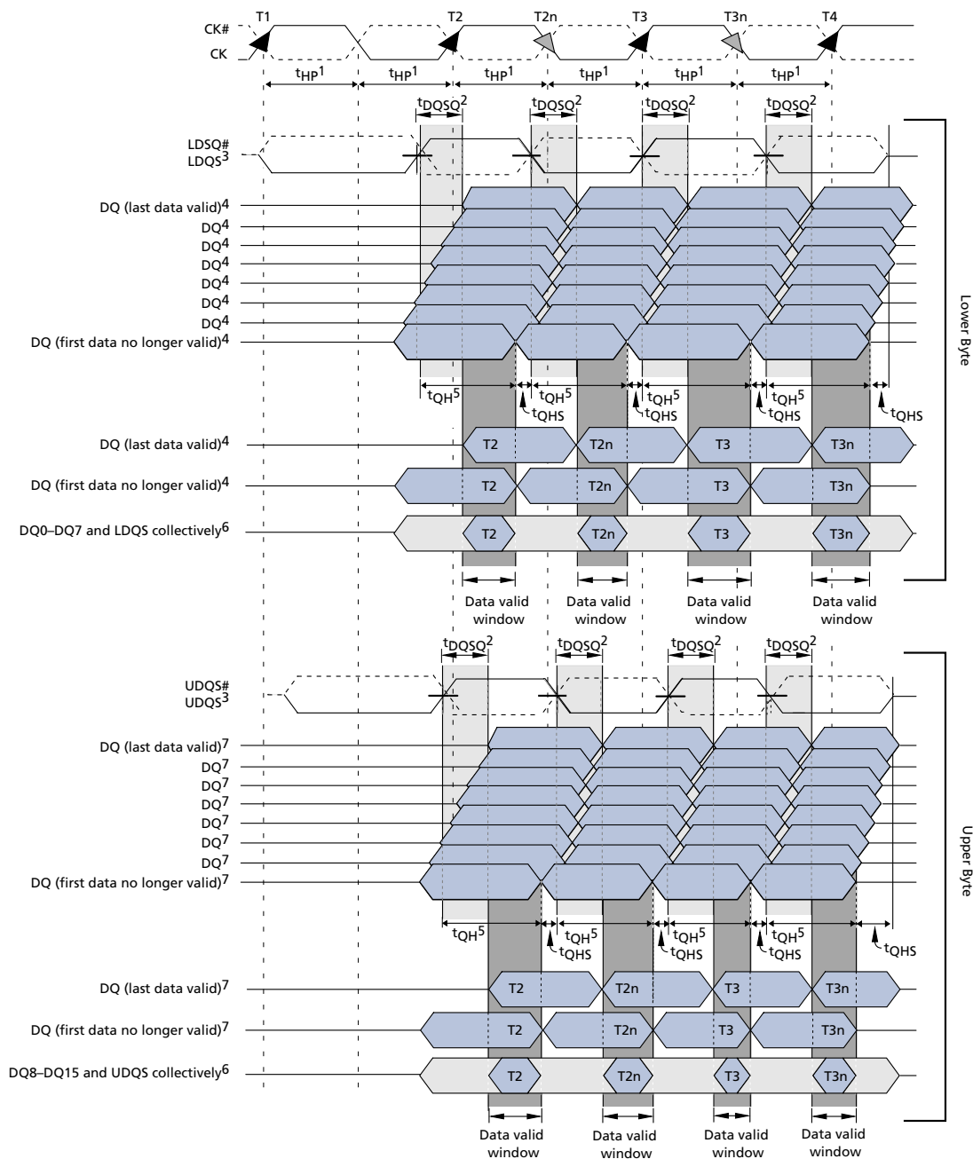
Figure 53: x16 Data Output Timing – t_{DQSQ} , t_{QH} , and Data Valid Window
