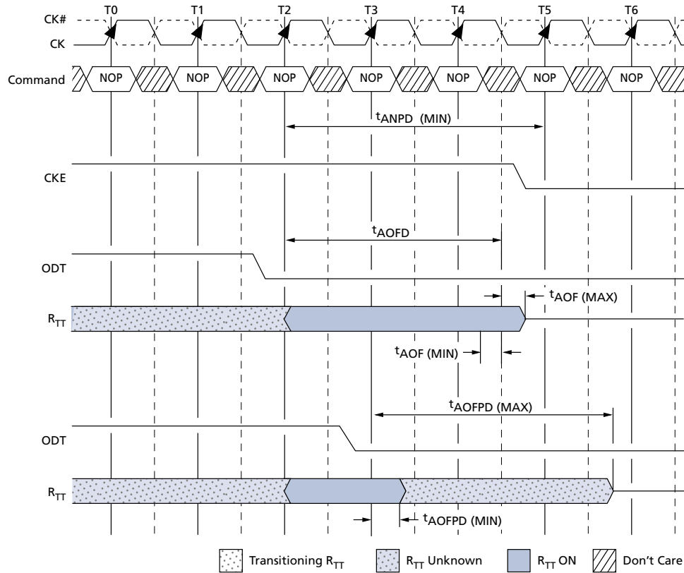
Figure 82: ODT Turn-Off Timings When Entering Power-Down Mode
