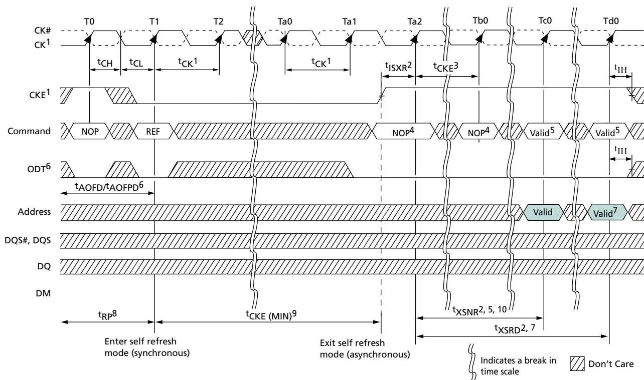
Figure 66: Self Refresh
