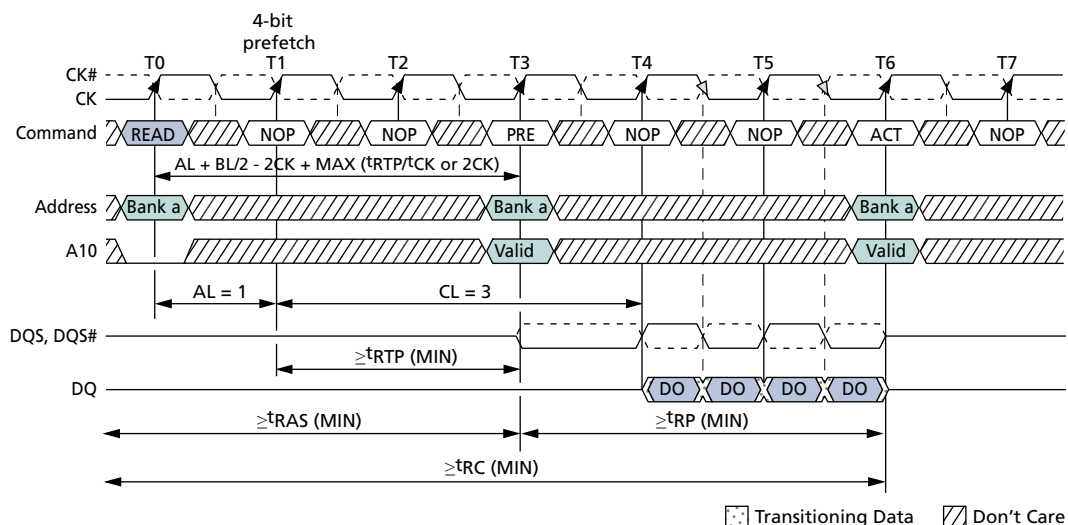
Figure 48: READ-to-PRECHARGE – BL = 4
