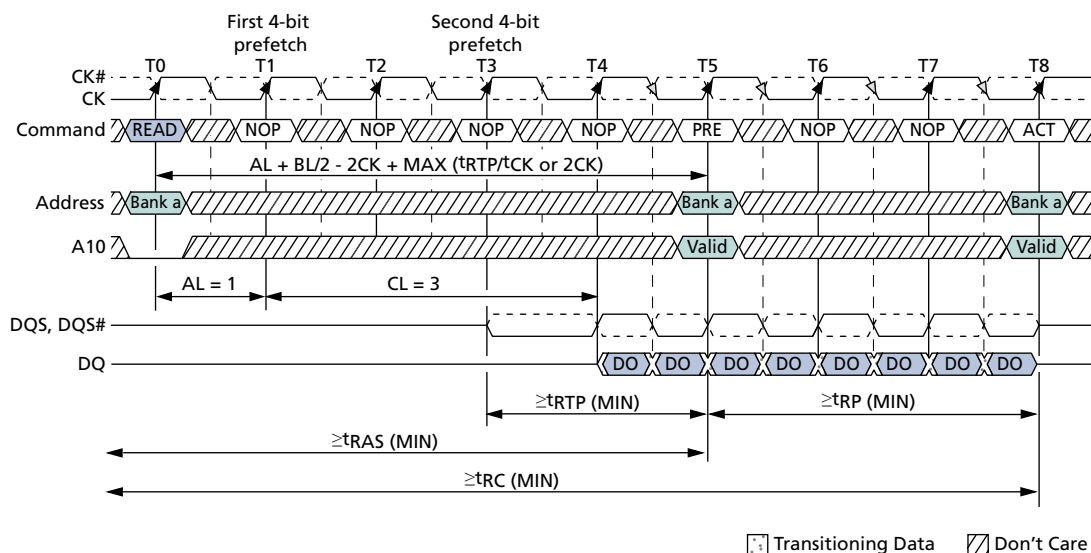
Figure 49: READ-to-PRECHARGE – BL = 8
