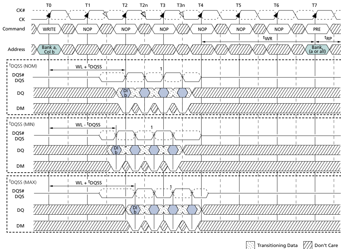
Figure 60: WRITE-to-PRECHARGE
