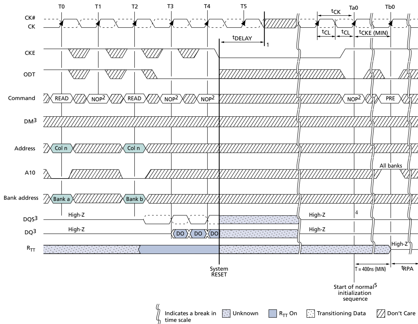
Figure 77: RESET Function
