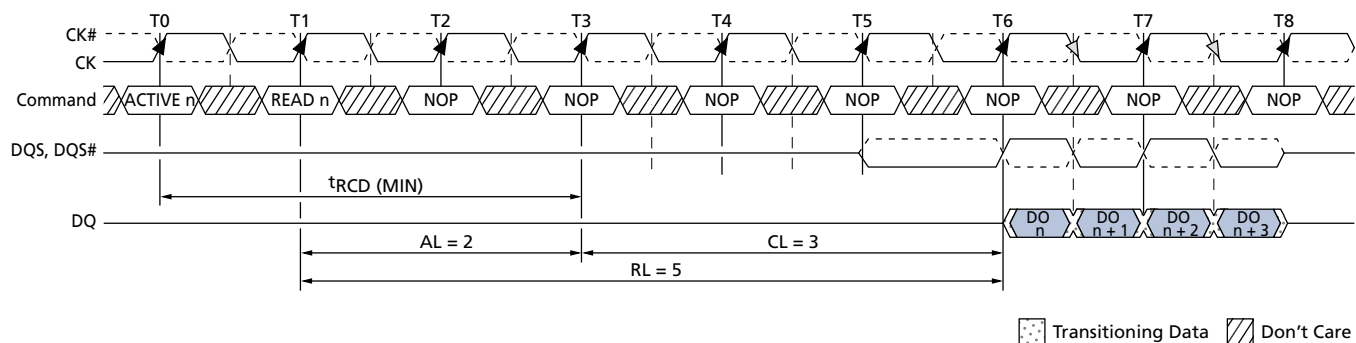
Figure 36: READ Latency
