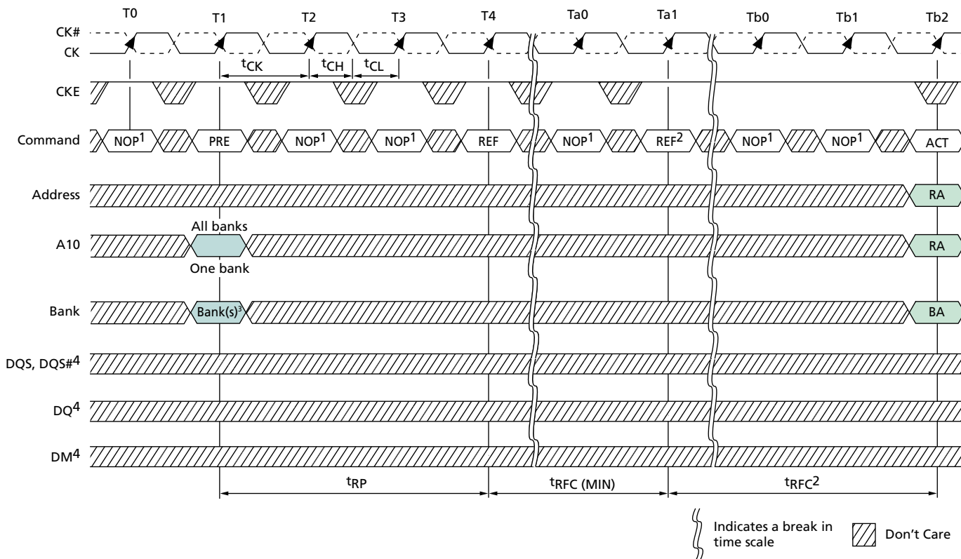
Figure 65: Refresh Mode
