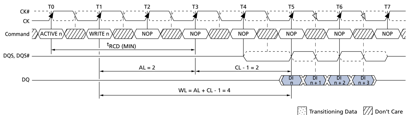
Figure 37: WRITE Latency
