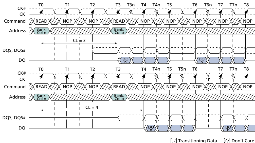
Figure 45: Nonconsecutive READ Bursts
