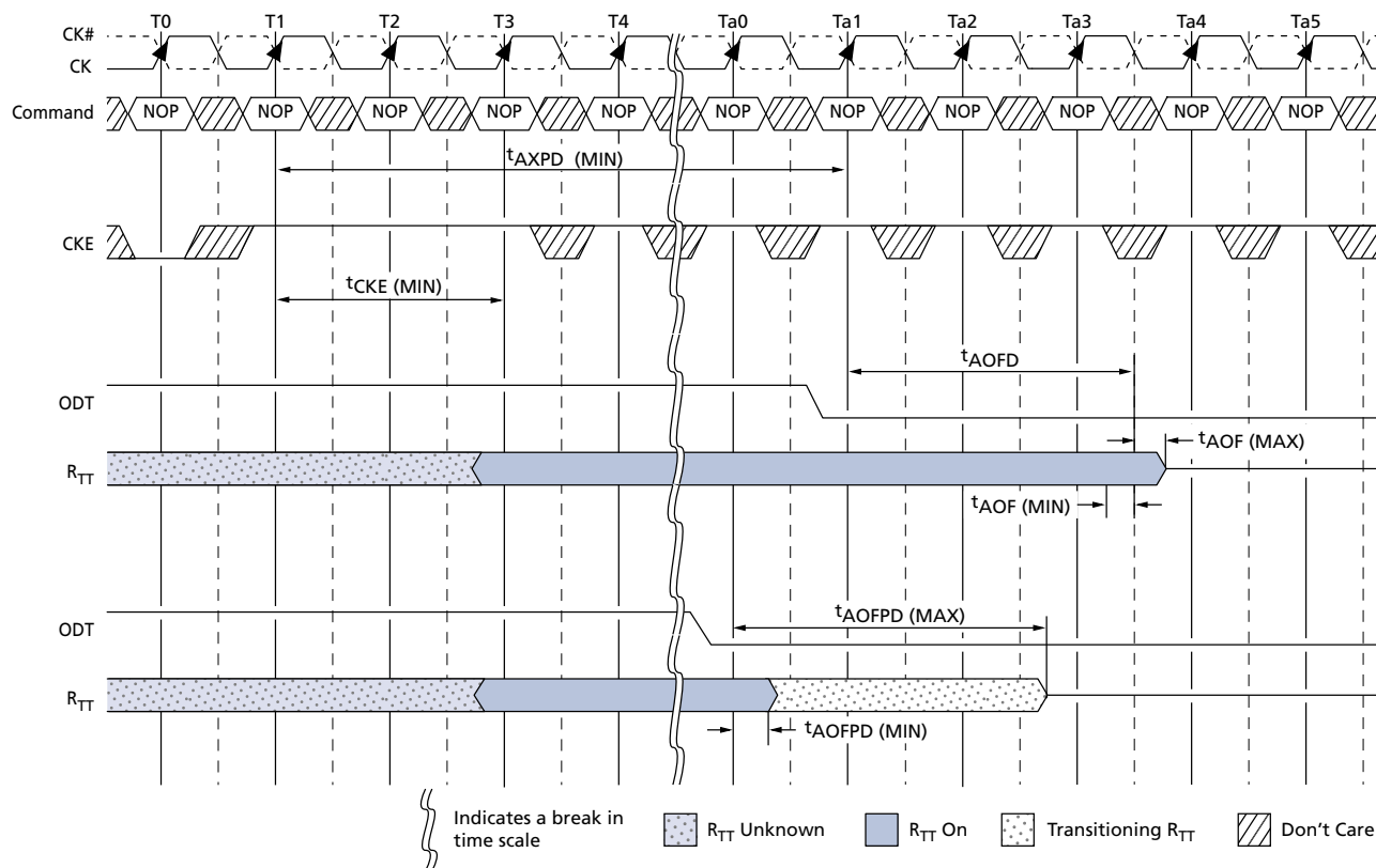
Figure 84: ODT Turn-Off Timing When Exiting Power-Down Mode
