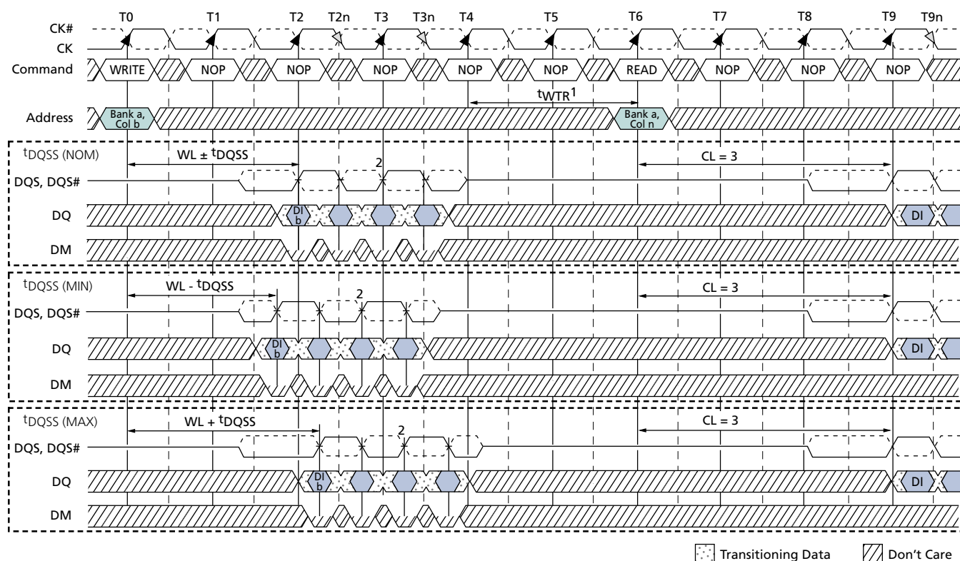
Figure 59: WRITE-to-READ
