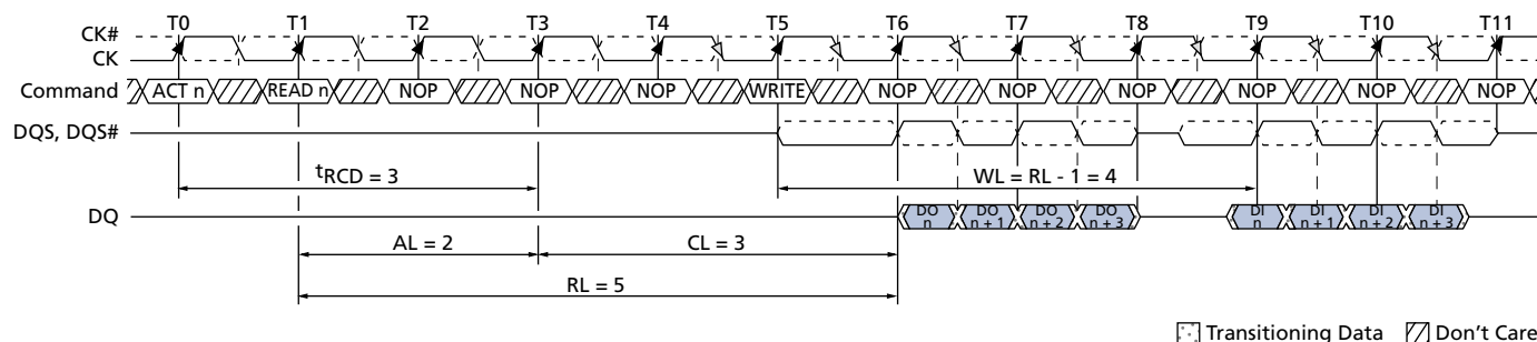
Figure 47: READ-to-WRITE
