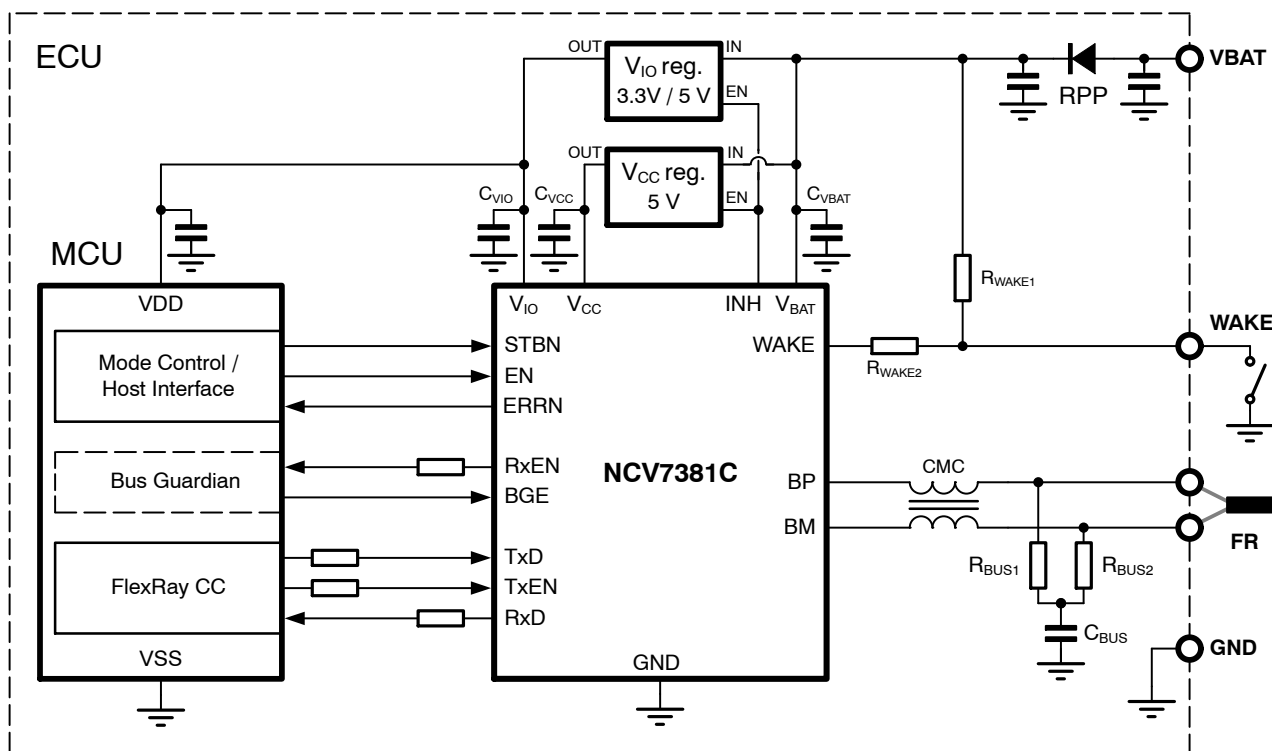
Figure 2. Application Diagram
