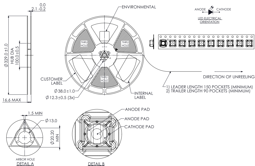
Figure 13a. Reel dimensions for L1I0-0xxx060000000, L1I0-0xxx090000000, and L1I0-0xxx955800000.
