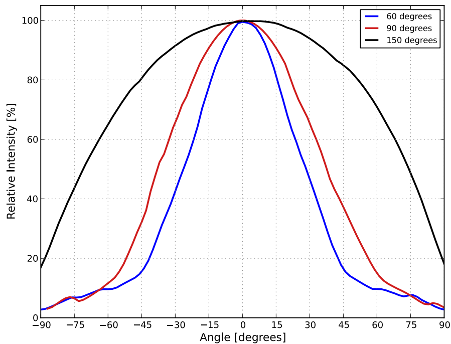
Figure 6a. Typical radiation pattern for L1I0-0xxx060000000, L1I0-0xxx090000000, and L1I0-0xxx150000000 at 1000mA, T j =25°C.
