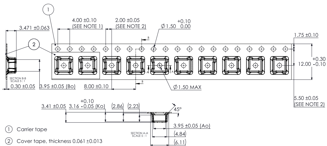
Figure 12a. Pocket tape dimensions for L110-0xxx0600000000.
