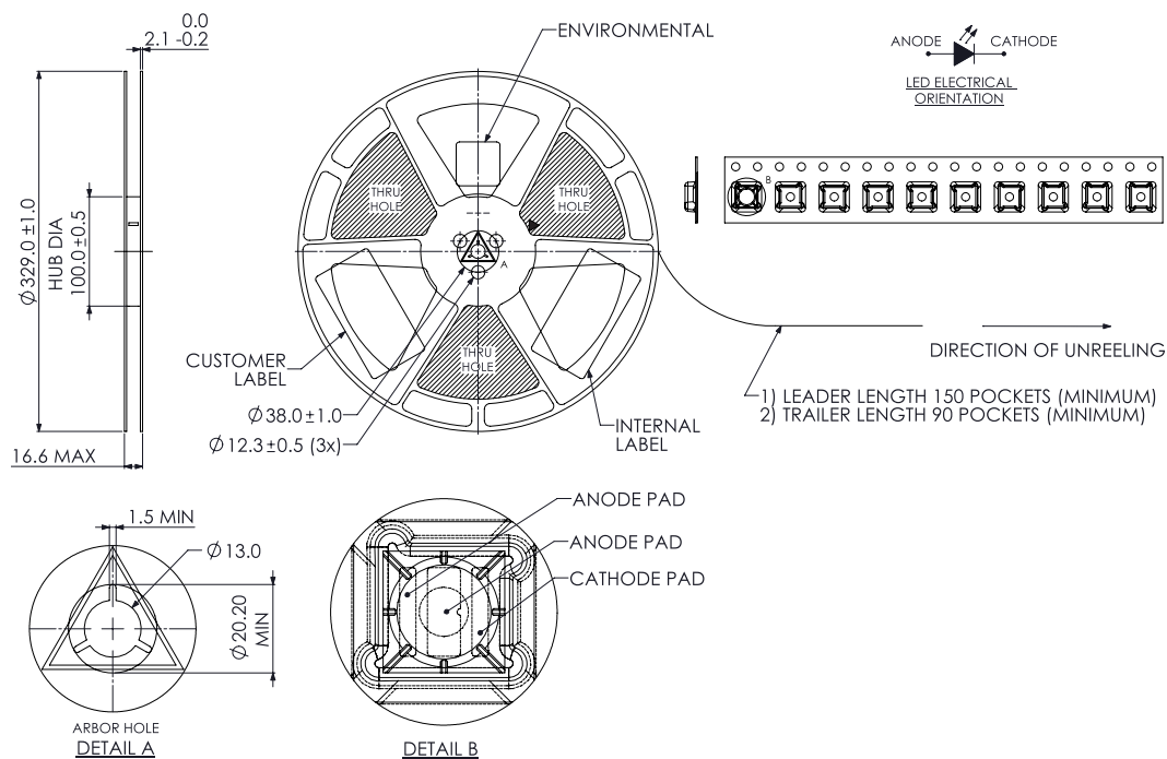
Figure 13b. Reel dimensions for L1I0-0xxx150000000.
