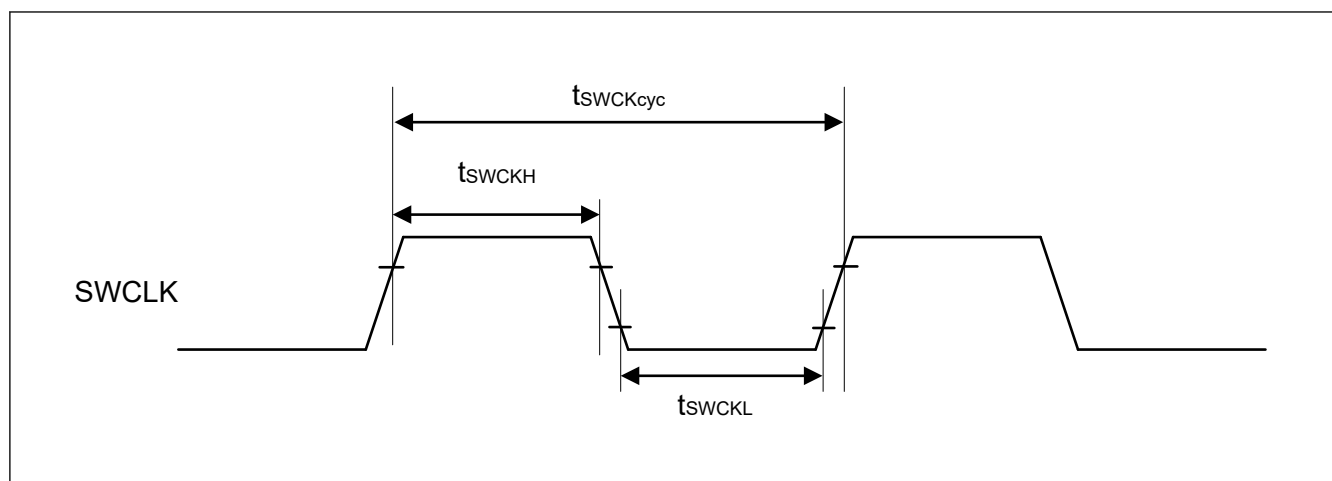
Figure 2.100 SWCLK timing
