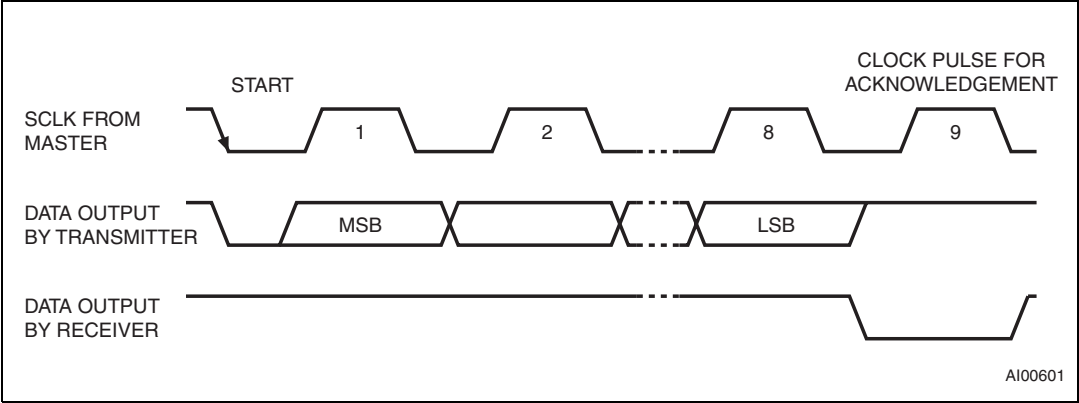
Figure 5. Acknowledge sequence
