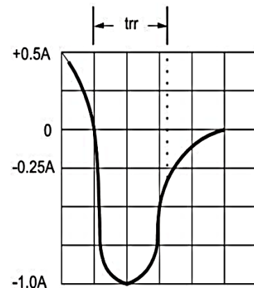
Fig.7 Reverse Recovery Time Characteristic And Test Circuit Diagram
