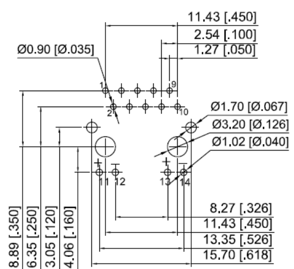
10 Pins, w/ LED For 100 PoE/1000/2.5G/5G Base-T
