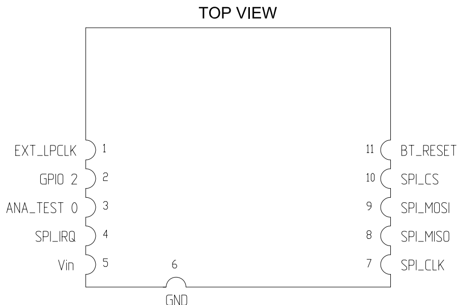
Figure 3. Pin connection
