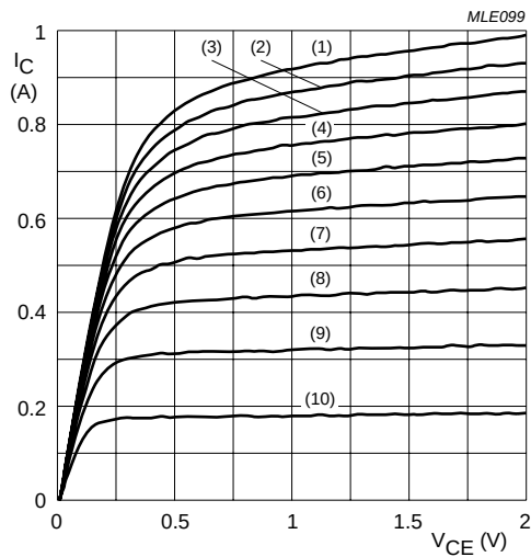
T_{amb} = 25\text{ }^{\circ}\text{C} . (1) I_B = 7\text{ mA} . (5) I_B = 4.2\text{ mA} . (9) I_B = 1.4\text{ mA} . (2) I_B = 6.3\text{ mA} . (6) I_B = 3.5\text{ mA} . (10) I_B = 0.7\text{ mA} . (3) I_B = 5.6\text{ mA} . (7) I_B = 2.8\text{ mA} . (4) I_B = 4.9\text{ mA} . (8) I_B = 2.1\text{ mA} .
